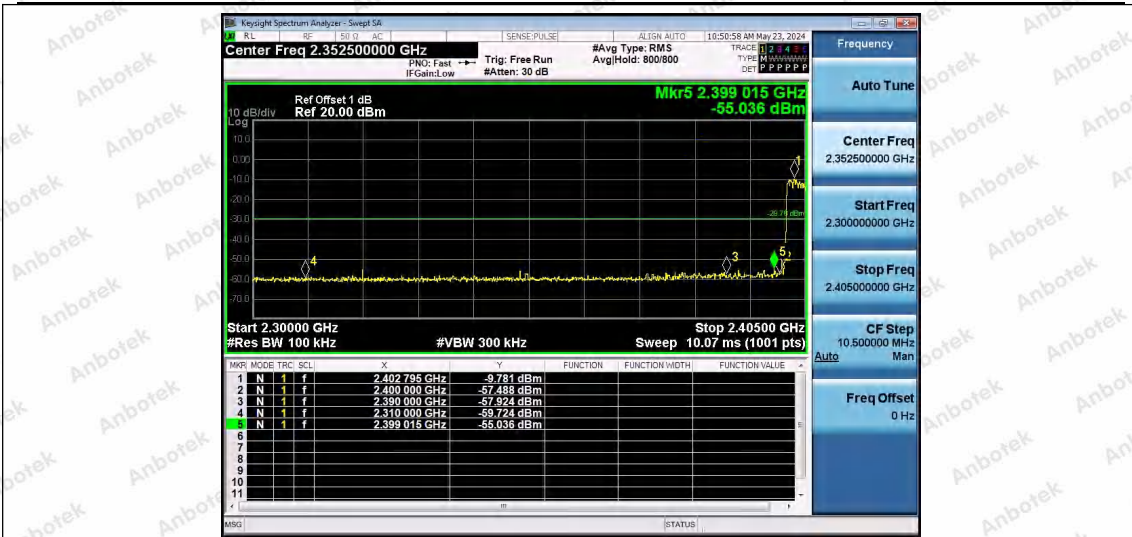
2DH5-Ant1-Hop_2402-PASS
