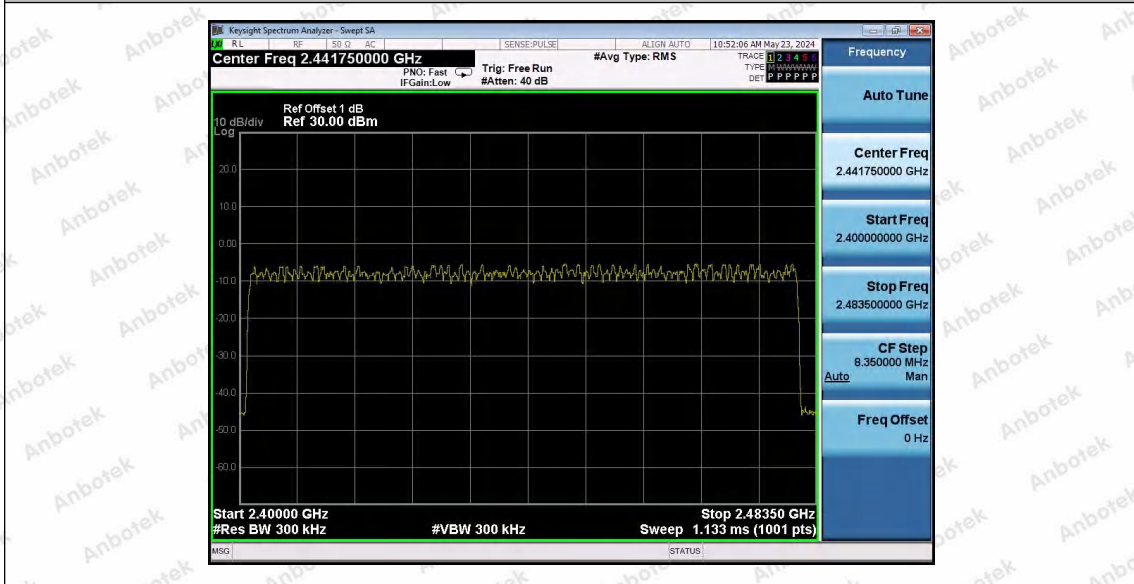
2DH5-Ant1-Hop-PASS
