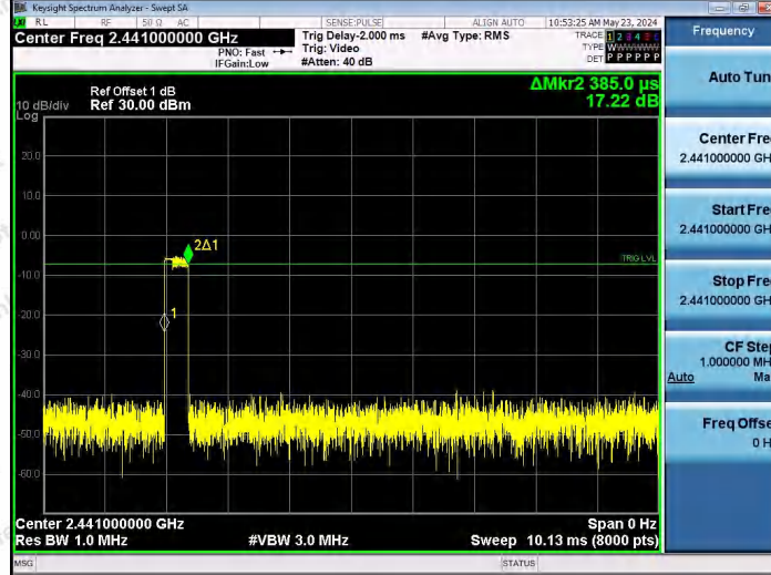
2DH1-Ant1-Hop-PASS
