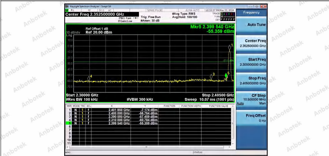
3DH5-Ant1-2402-PASS
