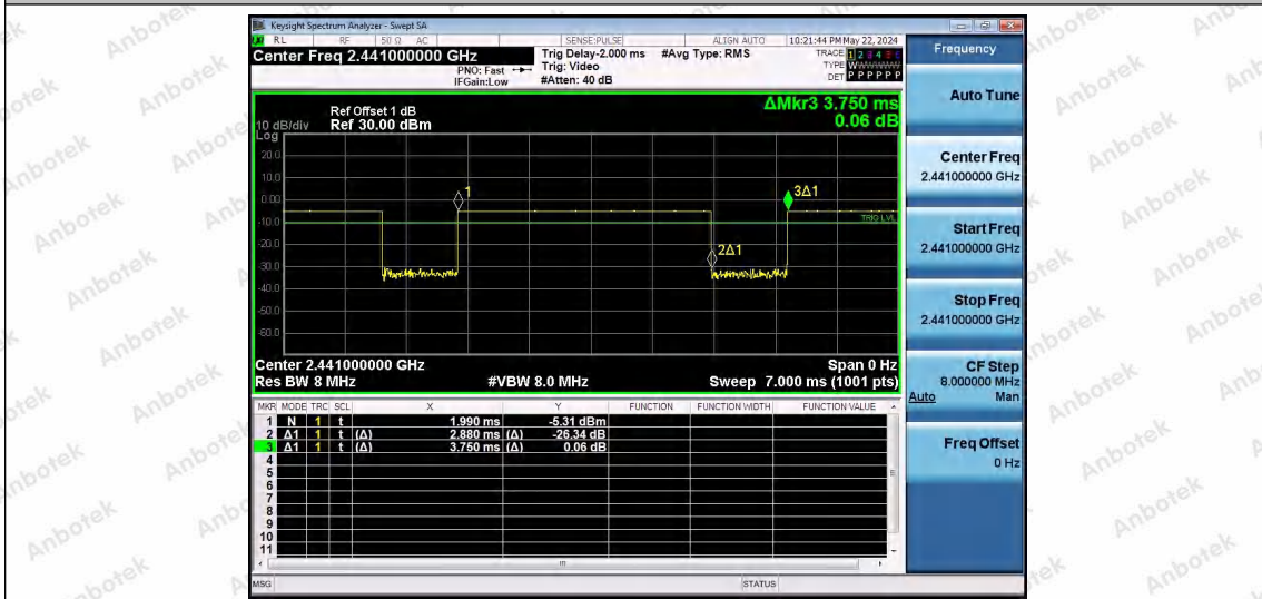
NTNV-DH5-Ant1-2441
