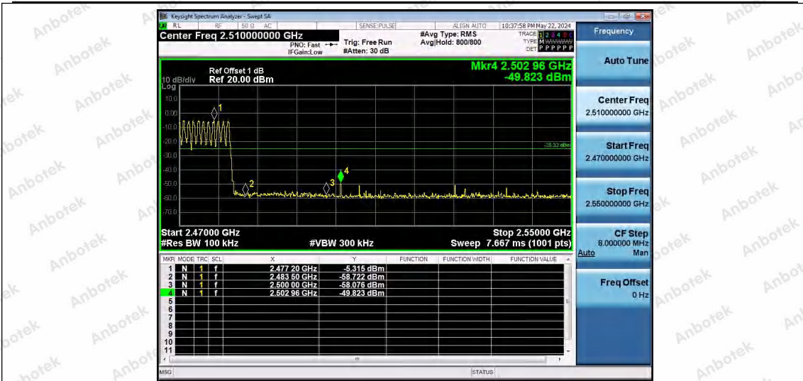
DH5-Ant1-Hop_2480-PASS
