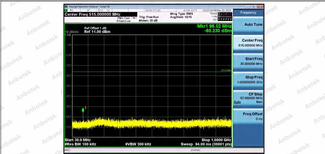
DH5-Ant1-2480-30~1000-PASS
