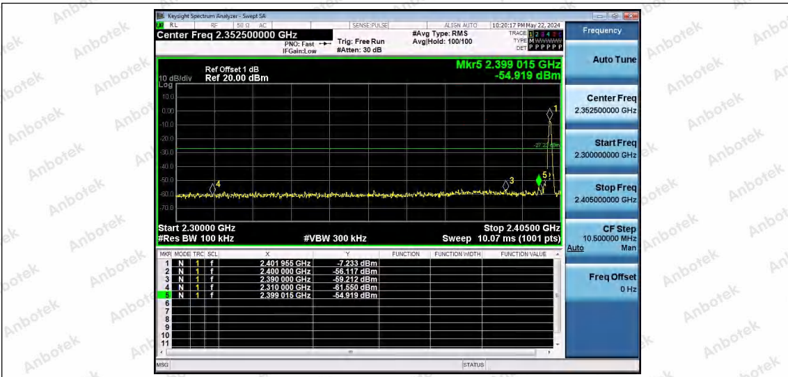
DH5-Ant1-2402-PASS
