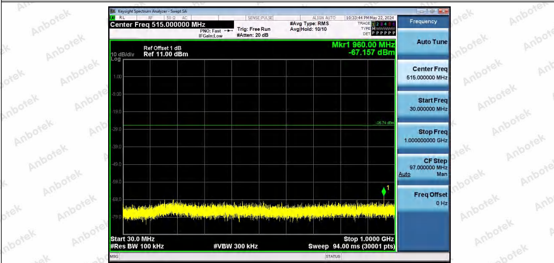
3DH5-Ant1-2402-30~1000-PASS
