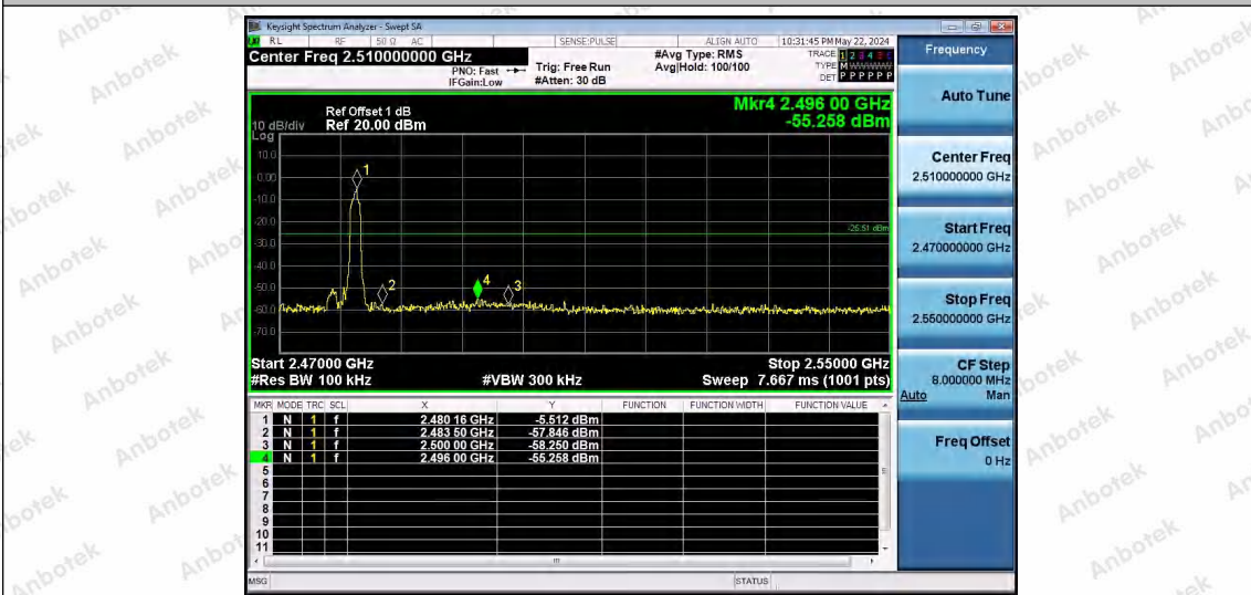
2DH5-Ant1-2480-PASS
