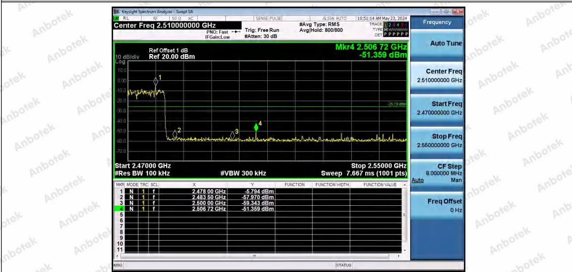
2DH5-Ant1-Hop_2480-PASS
