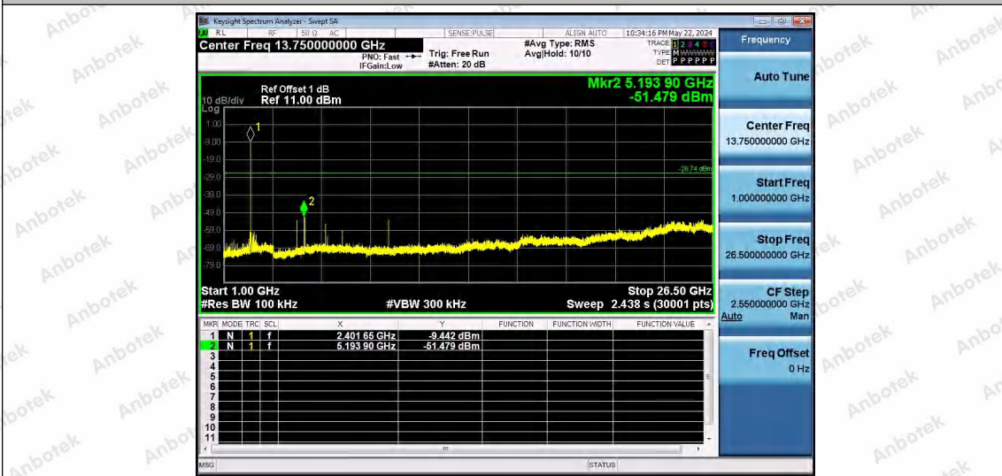
3DH5-Ant1-2402-1000~26500-PASS
