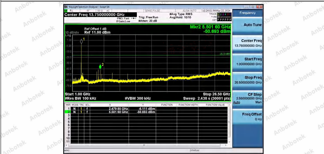
DH5-Ant1-2480-1000~26500-PASS
