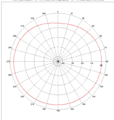
Far-field Power Distribution(H+V) on X-Y Plane Plot Peak Gain(H+V)= 1.35 dB; Plot AvgGain(H+V)= -0.83dB @2.44000 GHz
