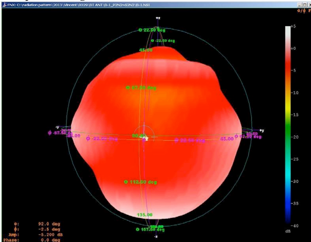
Far-field Power Distribution(H+V) on X-Y Plane Plot Peak Gain(H+V)= 1.35 dB; Plot AvgGain(H+V)= -0.83dB @2.44000 GHz
