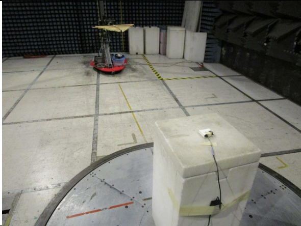
Spurious Emissions 200-1000 MHz
