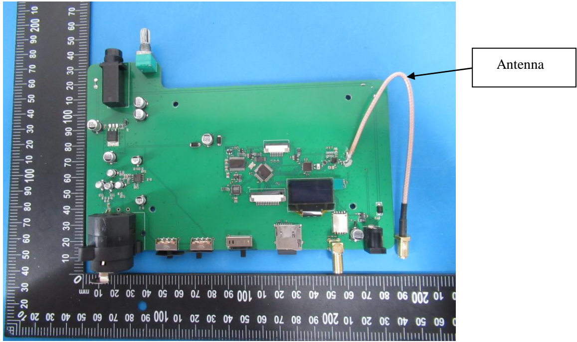
EUT View
