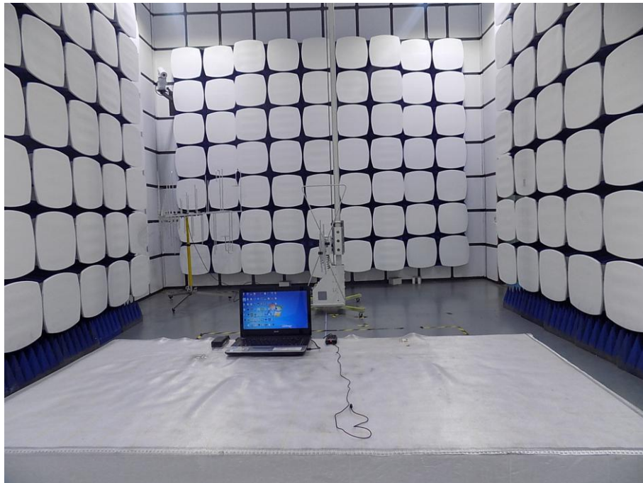
Photos of Radiated Emission Test (In Semi Anechoic Chamber)
