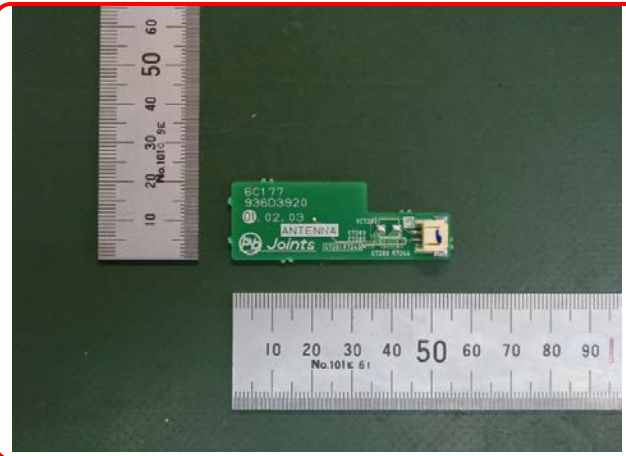
ANTENNA Surface
