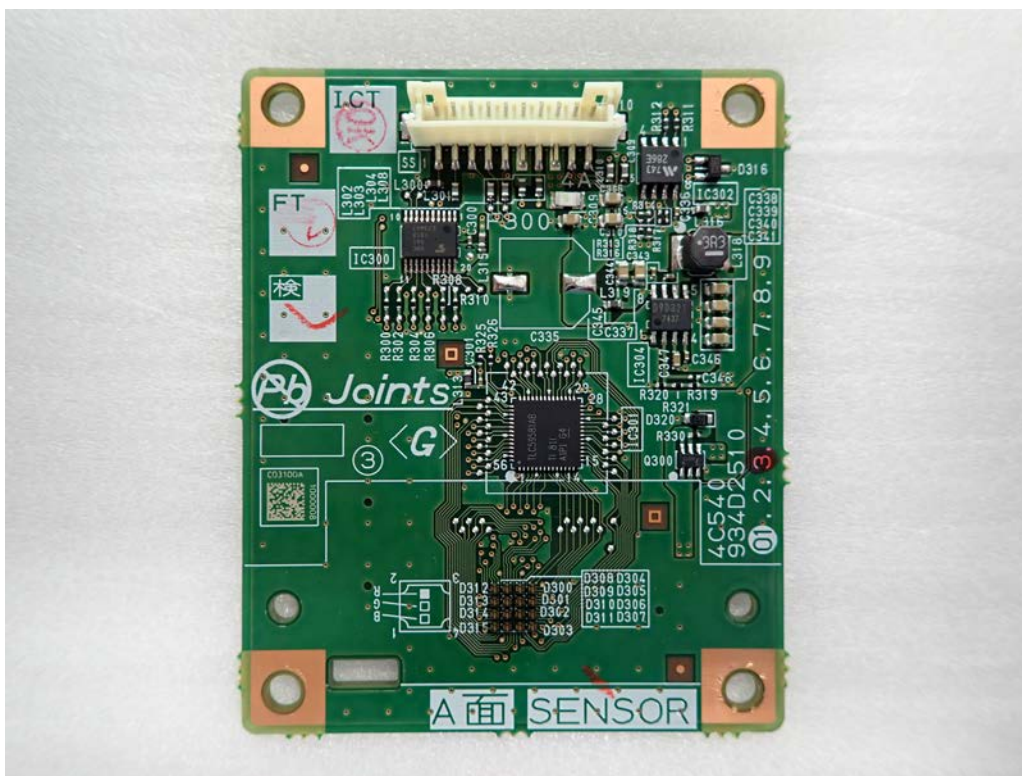
PWB-SENSOR-A
