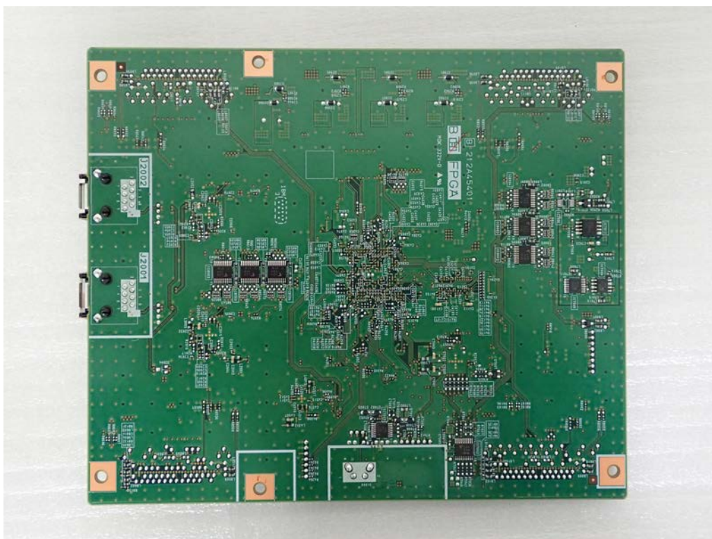
PWB-FPGA-B
