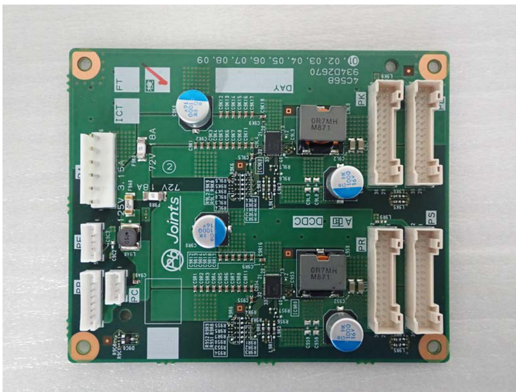
PWB-DCDC-A
