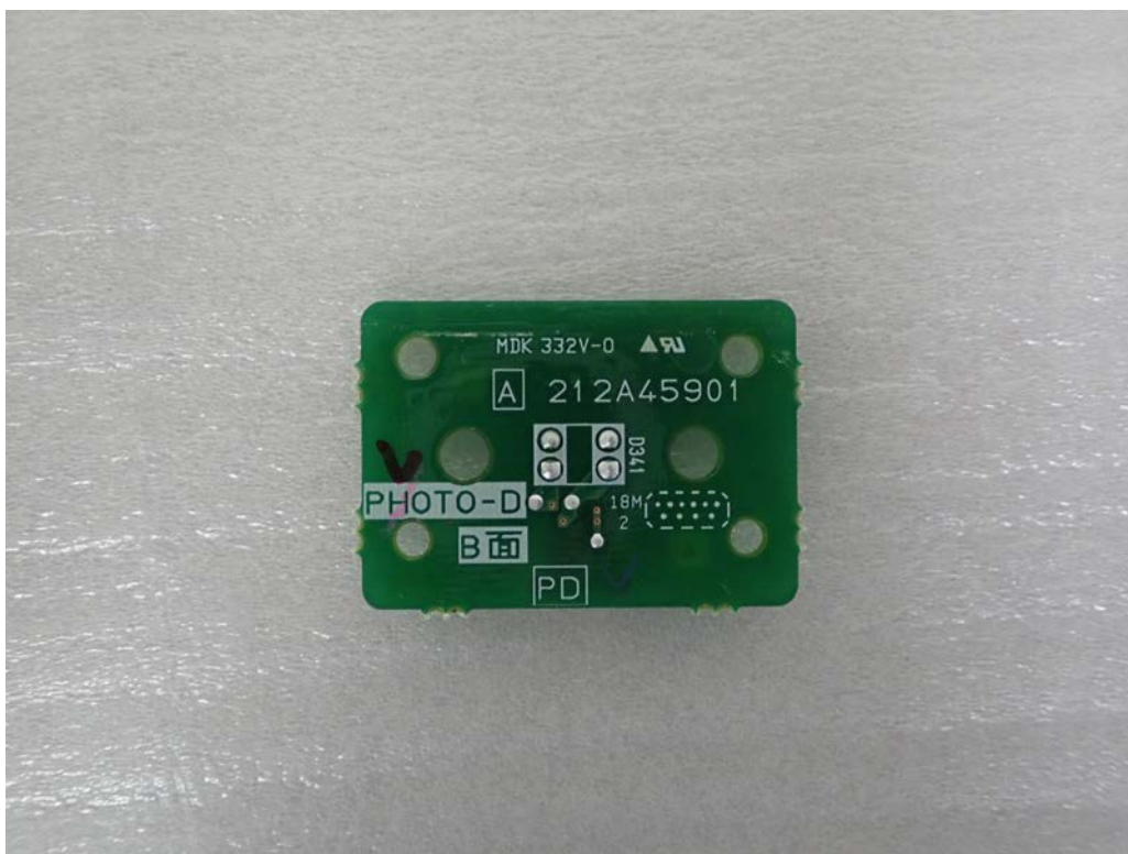
PHOTO-D-B
