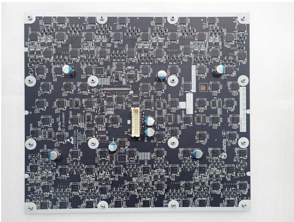
LEDPAN-B
