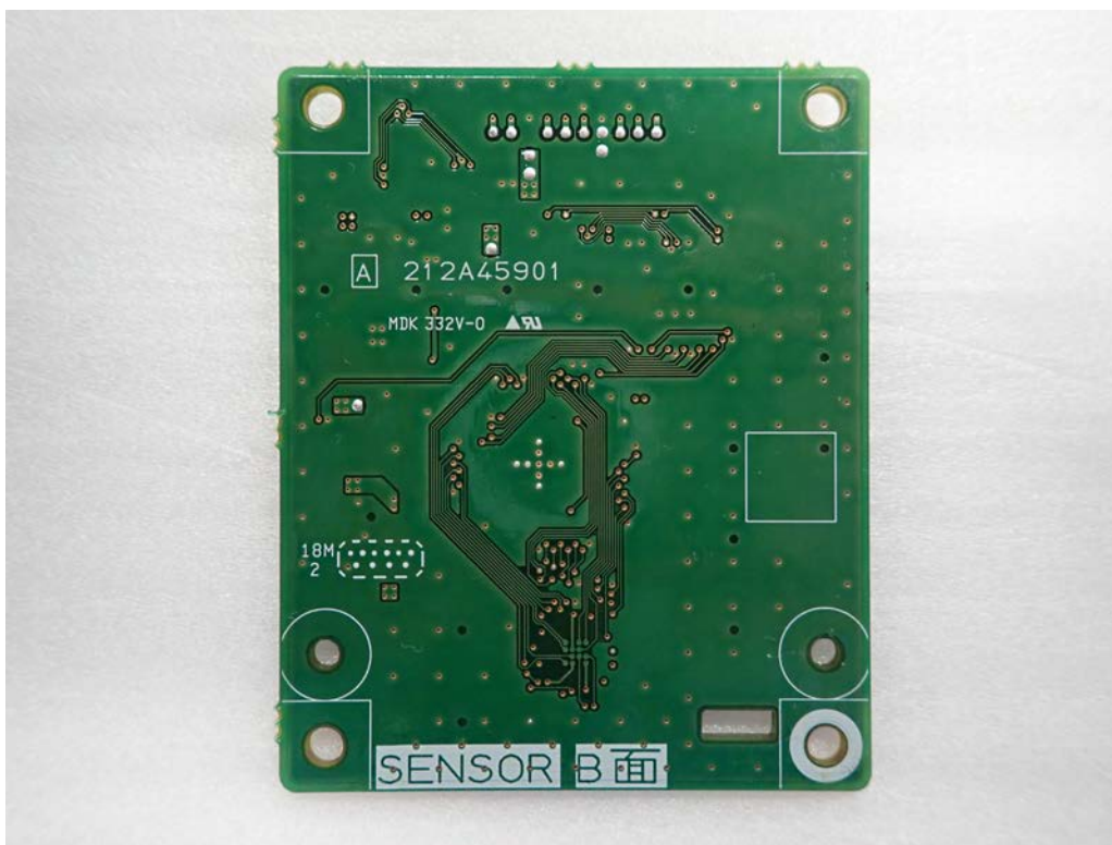
SENSOR-B
