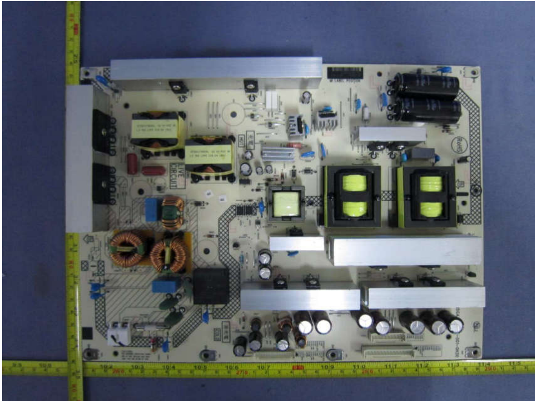
Figure 17 Frontside of Power Board
