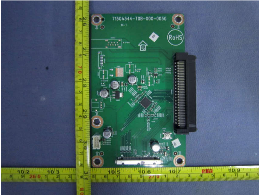
Figure 21 Frontside of PCB
