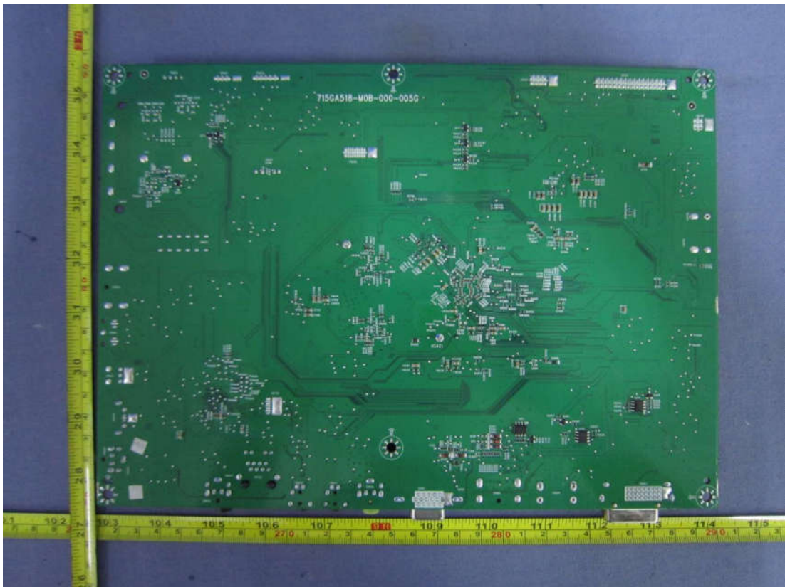
Figure 16 Backside of Main Board
