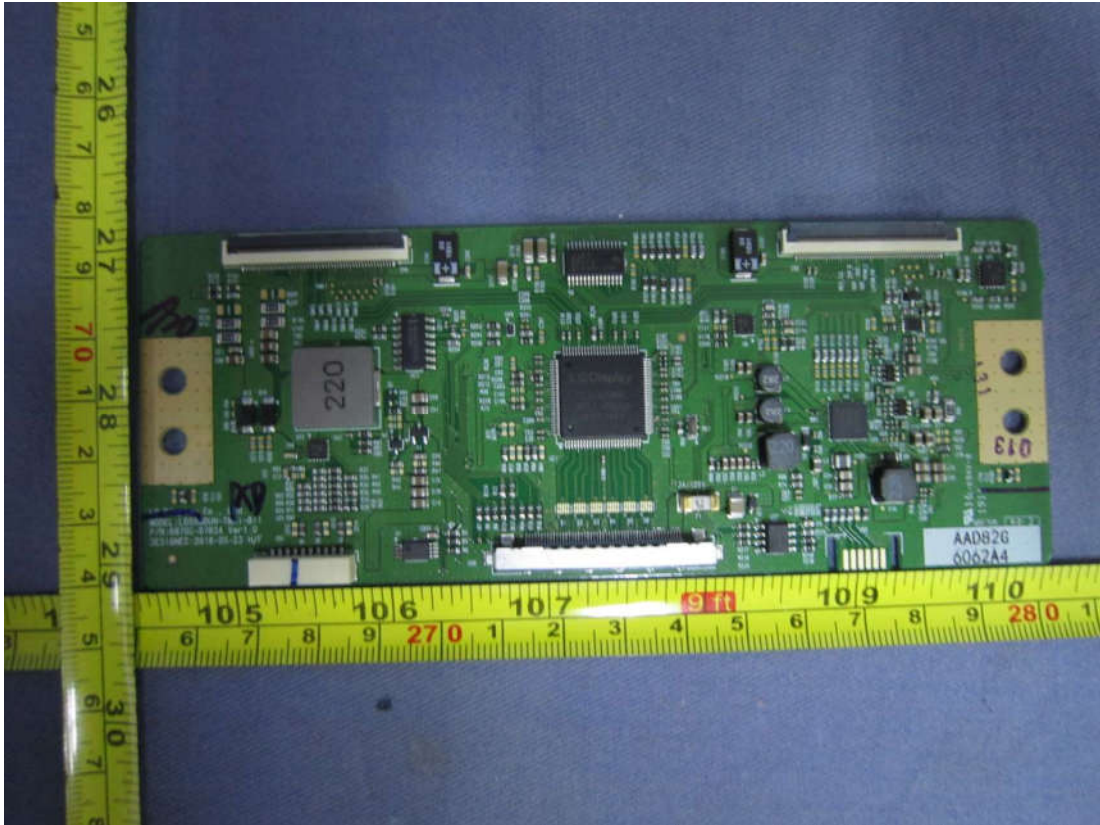
Figure 19 Frontside of PCB
