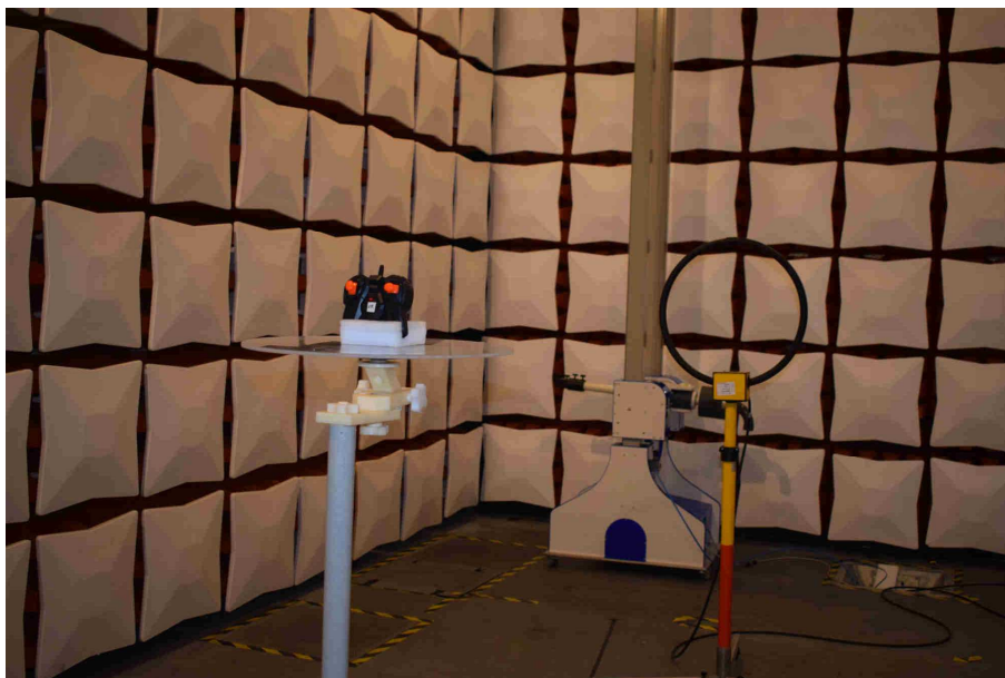
TX below 30MHz
