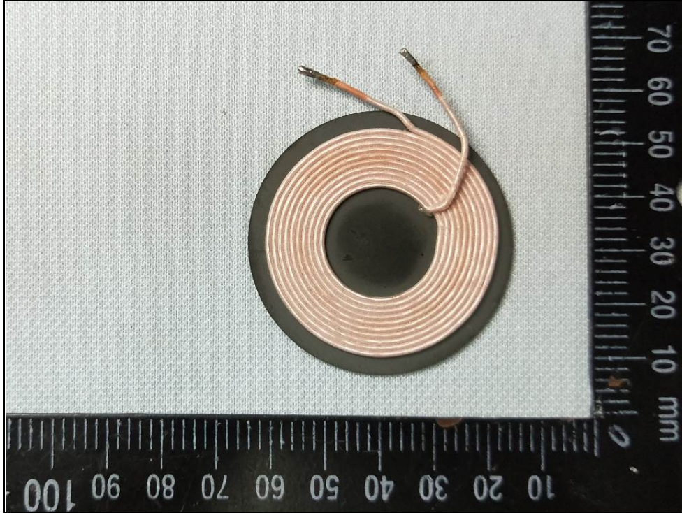
Induction coil
