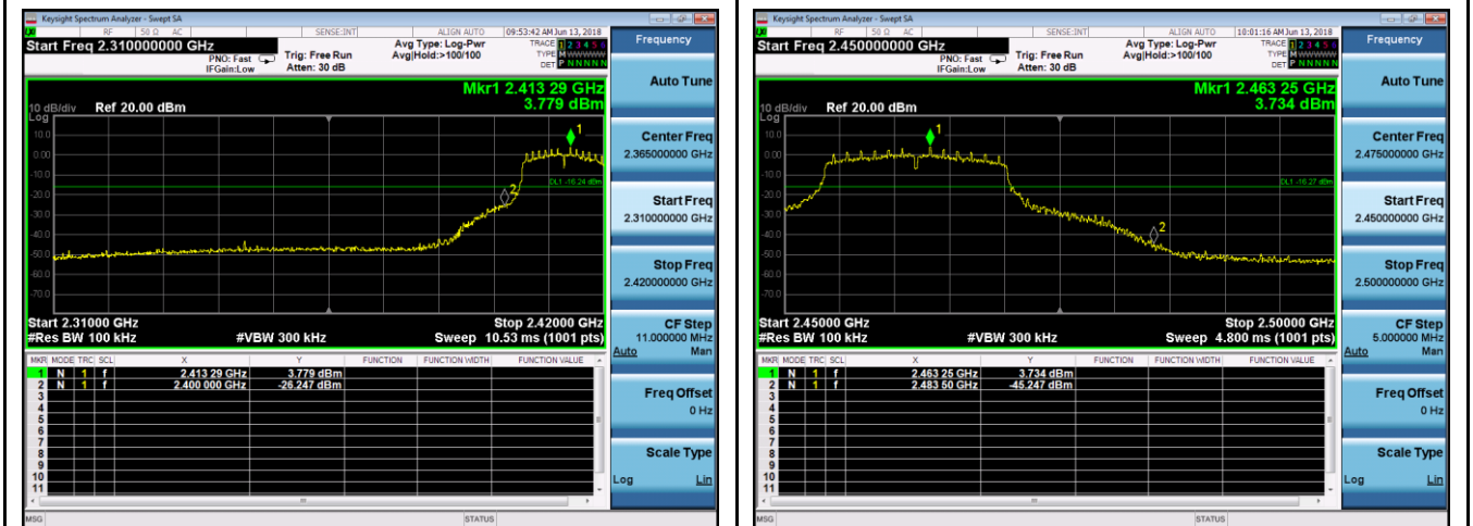
Band Edge, Left Side - 802.11g
