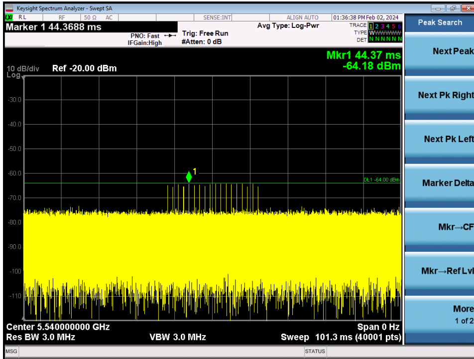
Radar Signal 0
