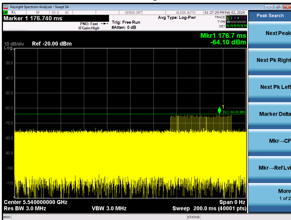
Radar Signal 1
