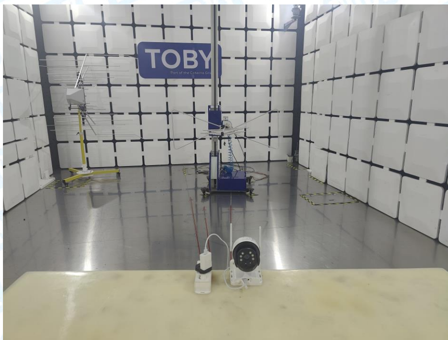
Photo of Setup for Radiated Emission (Below 1 GHz)-Q203A-G
