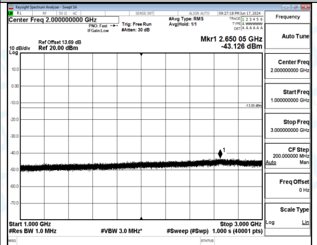
Band13_10MHz_16QAM_23230_1RB#49_1000-3000_1000-3000
