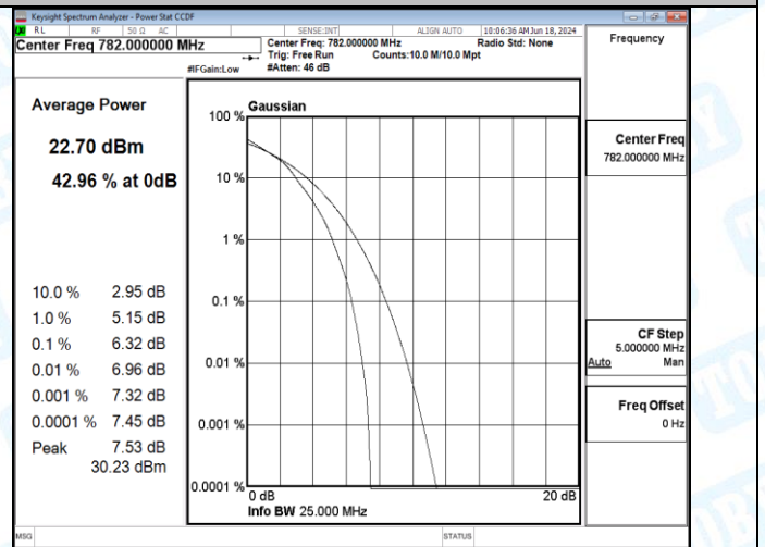
Band13-10MHz-16QAM-23230-27RB#0-PASS
