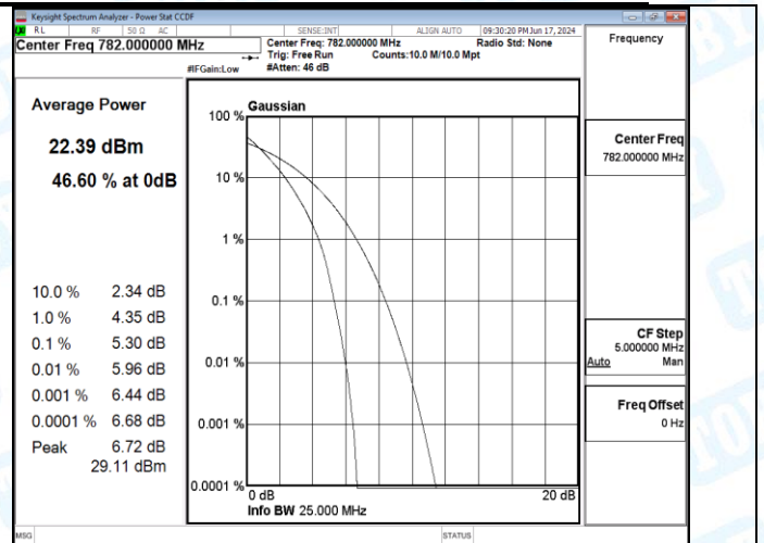
Band13-10MHz-16QAM-23230-27RB#0-PASS
