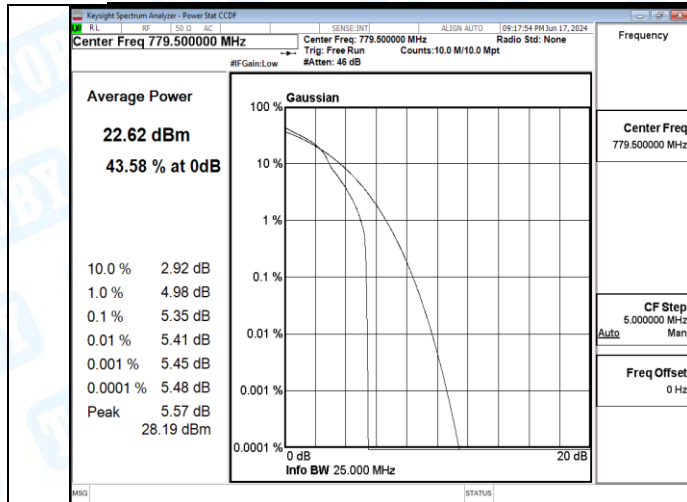
Band13-5MHz-16QAM-23230-1RB#0-PASS
