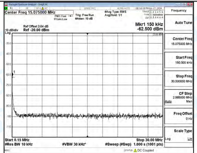
Band12_10MHz_QPSK_23130_50RB#0_1000~3000_1000~3000
