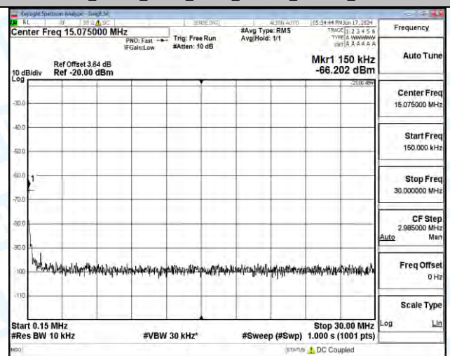
Band5_10MHz_QPSK_20525_1RB#49_1000~3000_1000~3000
