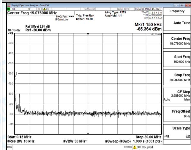
Band12_3MHz_16QAM_23025_15RB#0_1000~3000_1000~3000
