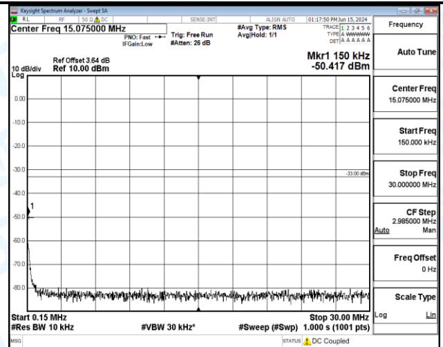
Band66_10MHz_16QAM_132322_1RB#49_1000~3000_1000~3000
