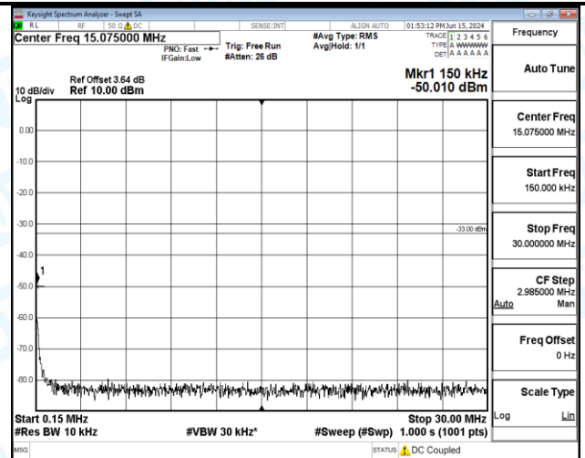
Band66_15MHz_16QAM_132047_1RB#0_1000~3000_1000~3000
