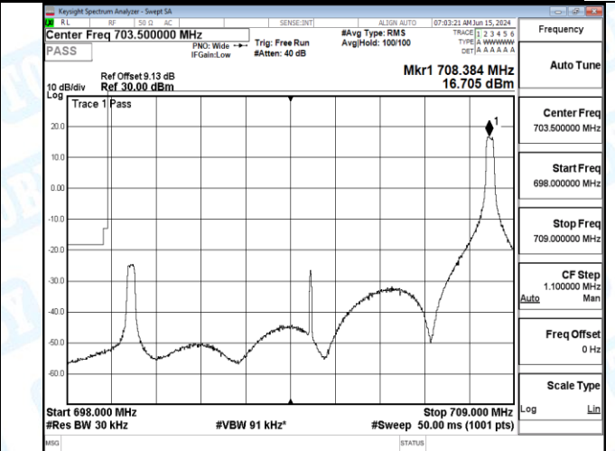
Band12_10MHz_QPSK_23130_1RB#0
