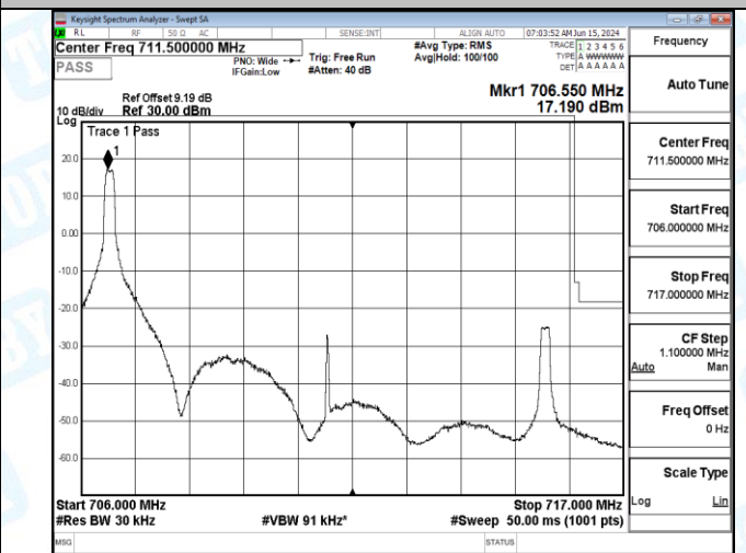
Band12_10MHz_QPSK_23130_50RB#0
