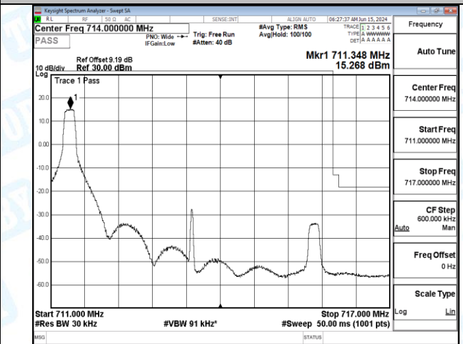
Band12_5MHz_16QAM_23155_25RB#0
