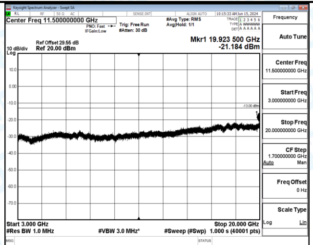
Band66_5MHz_QPSK_132322_1RB#24_0.15~30_0.15~30
