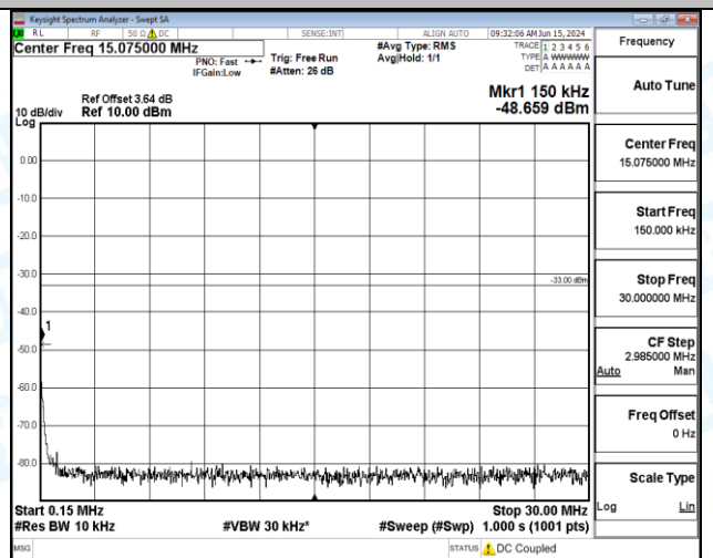
Band66_3MHz_16QAM_132322_15RB#0_1000-3000_1000-3000
