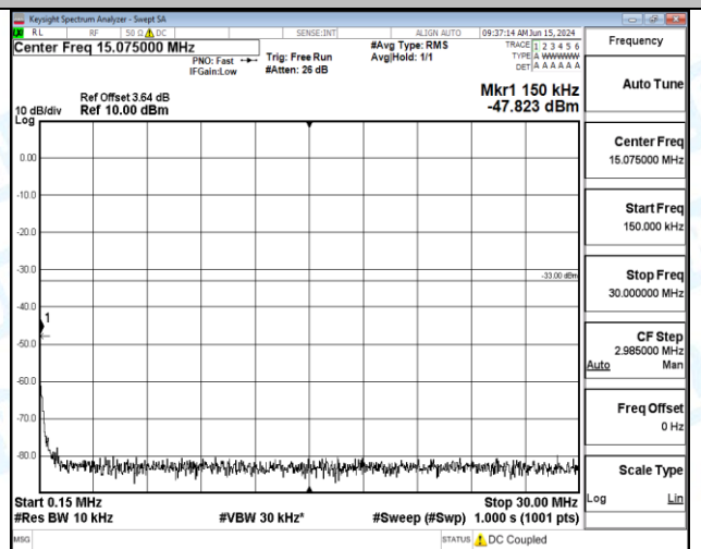
Band66_3MHz_QPSK_132657_15RB#0_1000~3000_1000~3000
