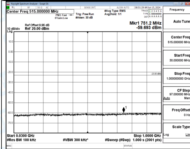
Band66_1.4MHz_16QAM_132322_6RB#0_3000~20000_3000~20000
