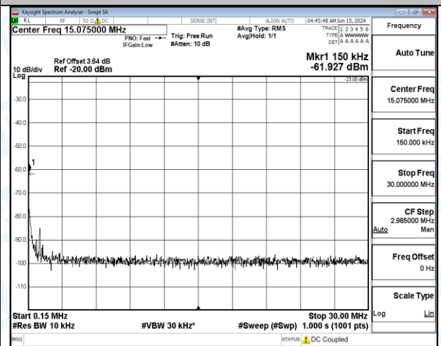
Band5_10MHz_QPSK_20525_1RB#49_1000~3000_1000~3000
