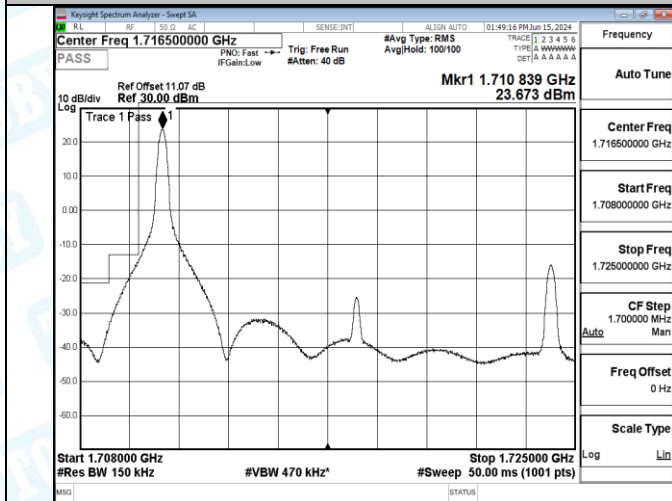
Band66_15MHz_QPSK_132047_75RB#0
