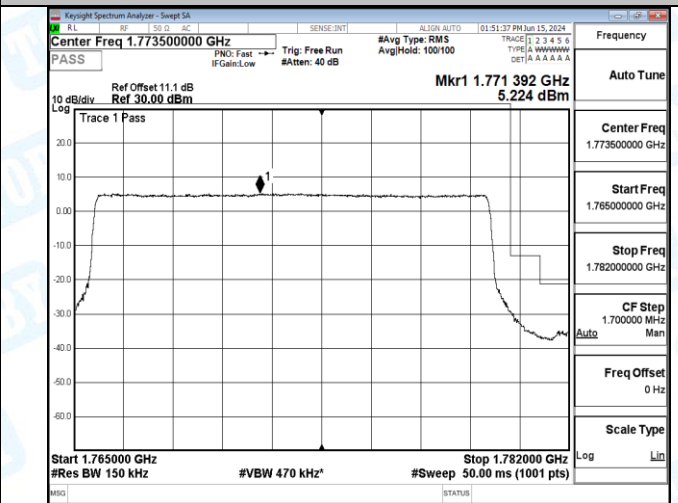
Band66_15MHz_QPSK_132597_75RB#0
