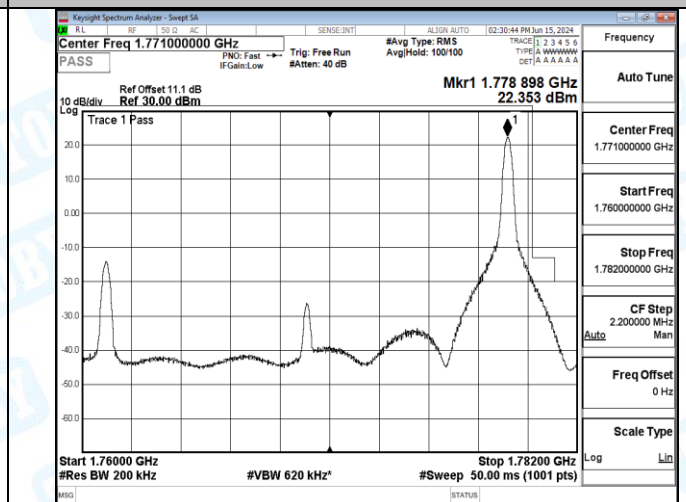
Band66_20MHz_16QAM_132572_1RB#99
