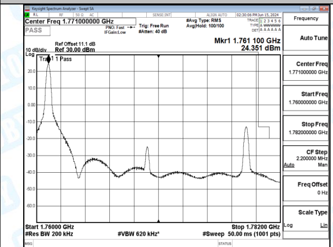
Band66_20MHz_QPSK_132572_100RB#0
