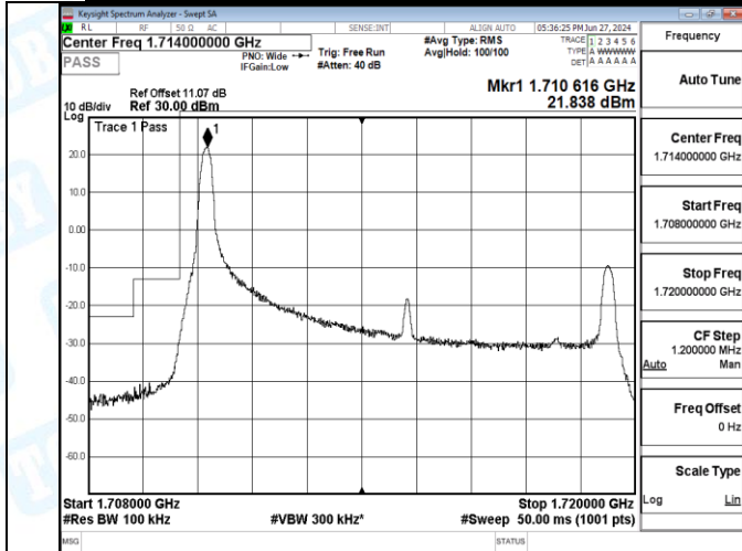
Band66_10MHz_16QAM_132622_1RB#0
