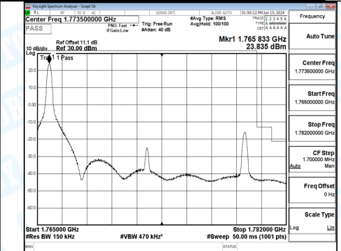
Band66_15MHz_QPSK_132597_75RB#0
