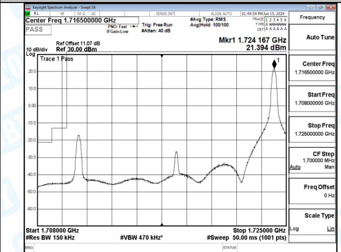
Band66_15MHz_16QAM_132047_1RB#74
