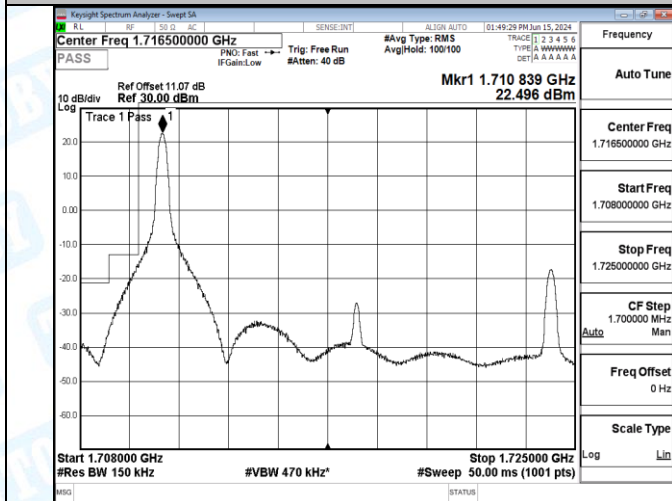
Band66_15MHz_16QAM_132047_1RB#0
