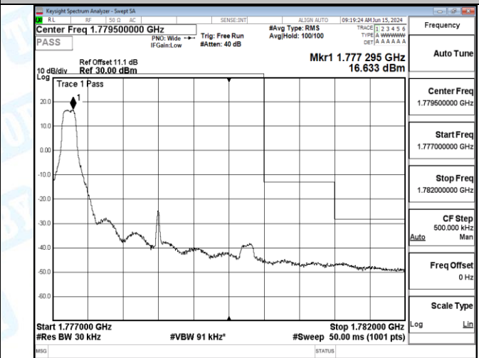
Band66_3MHz_QPSK_132657_15RB#0
