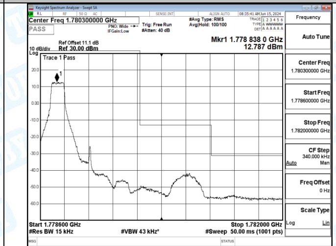
Band66_1.4MHz_16QAM_132665_6RB#0
