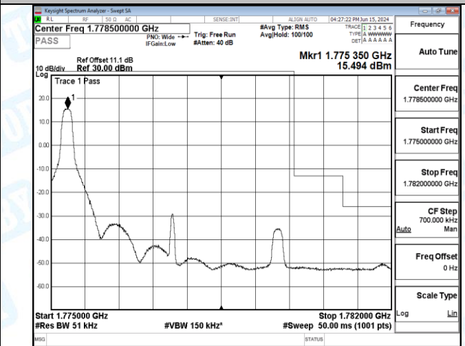
Band66_5MHz_16QAM_132647_25RB#0
