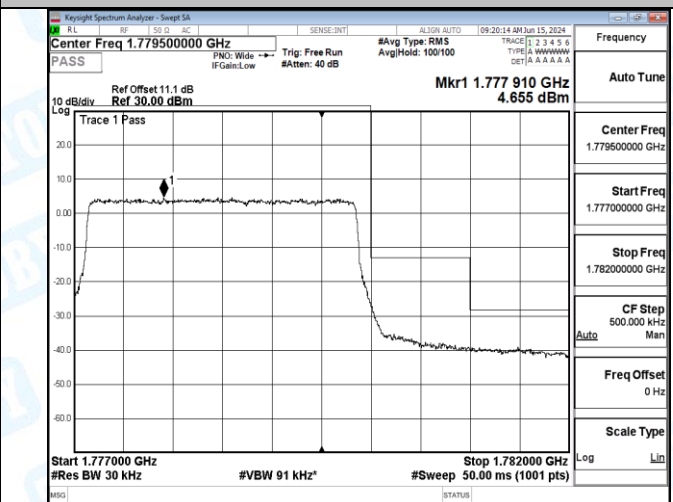
Band66_3MHz_16QAM_131987_1RB#14
