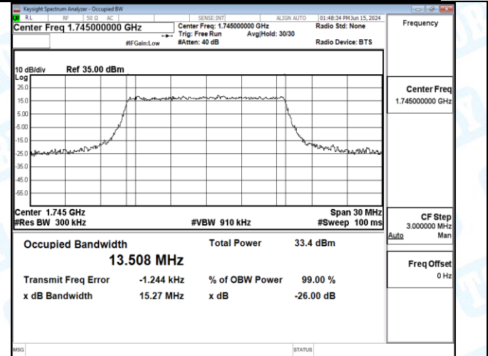
Band66-15MHz-16QAM-132047-27RB#0-PASS
