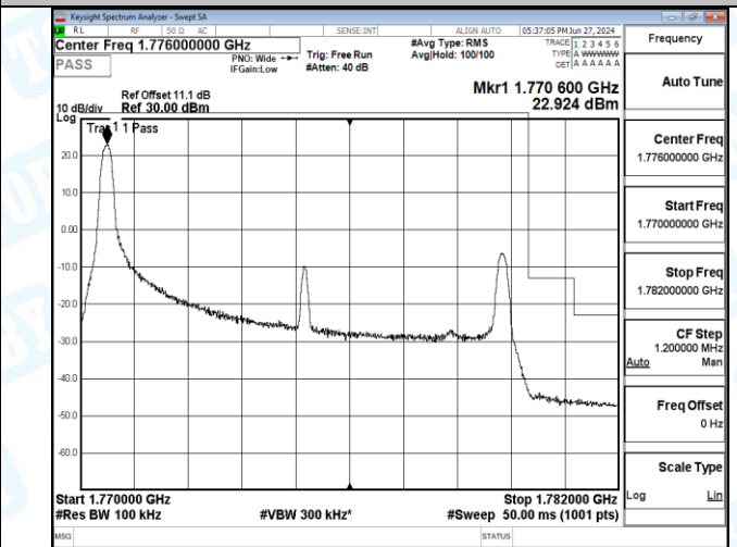
Band66_10MHz_QPSK_132622_50RB#0
