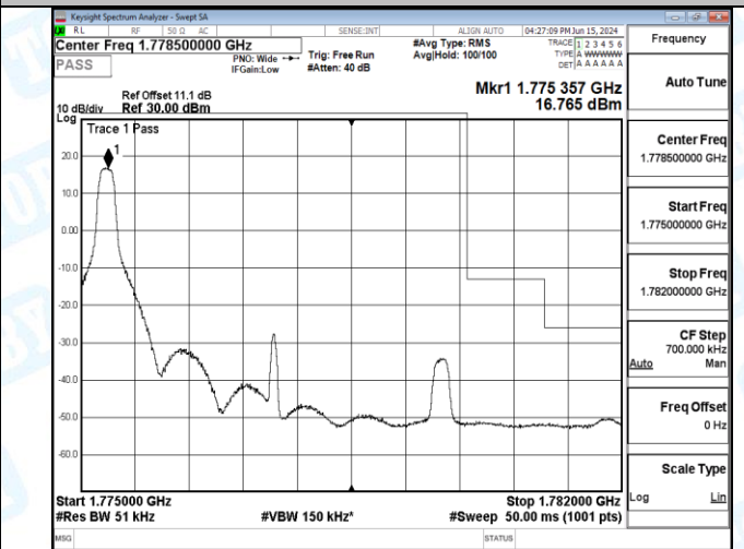
Band66_5MHz_QPSK_132647_25RB#0
