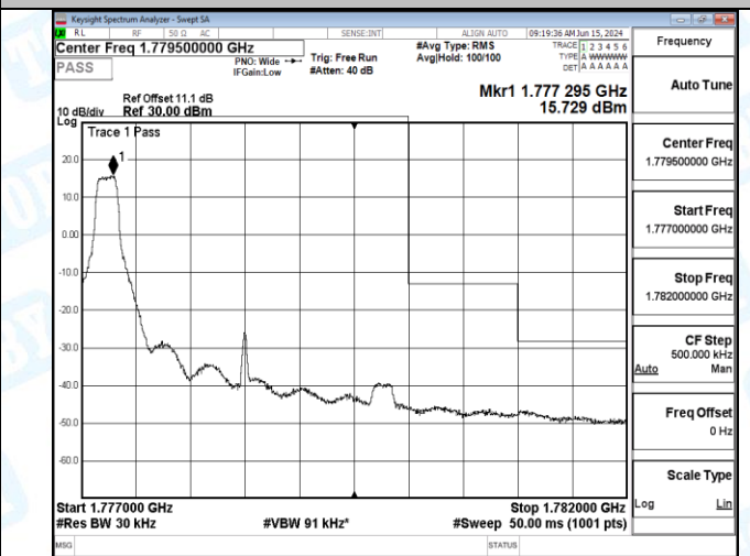
Band66_3MHz_16QAM_132657_15RB#0
