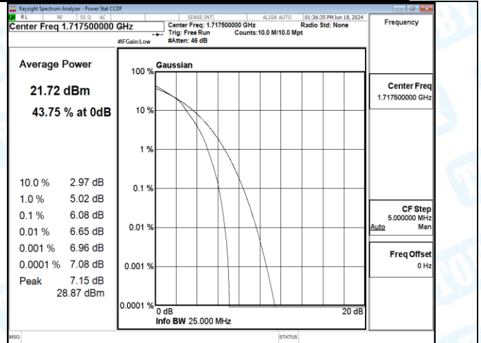
Band66-15MHz-16QAM-132322-27RB#0-PASS
