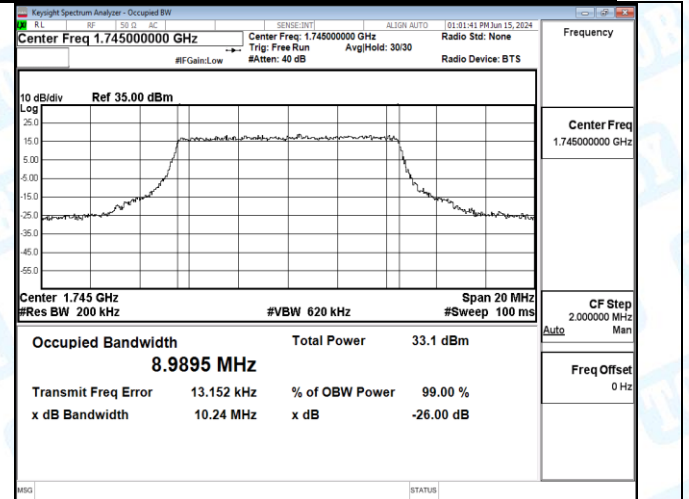
Band66-10MHz-16QAM-132022-27RB#0-PASS
