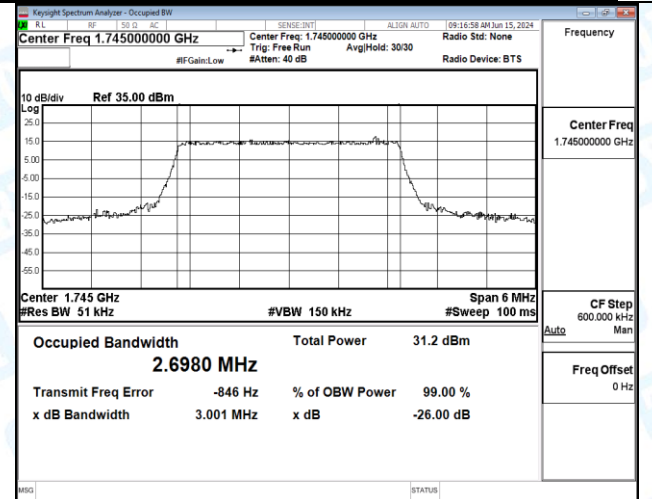
Band66-3MHz-16QAM-131987-15RB#0-PASS
