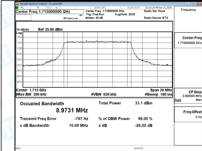
Band66-10MHz-QPSK-132622-50RB#0-PASS
