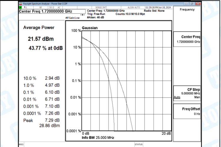
Band66-20MHz-16QAM-132322-27RB#0-PASS
