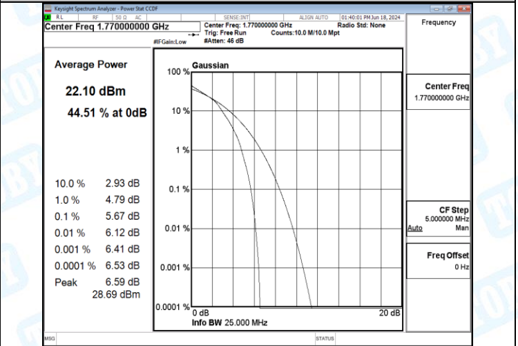
Band66-20MHz-16QAM-132572-27RB#0-PASS
