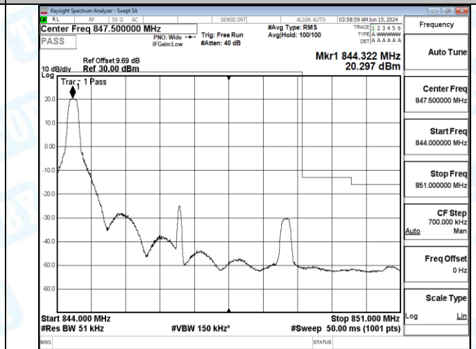
Band5_5MHz_QPSK_20625_25RB#0
