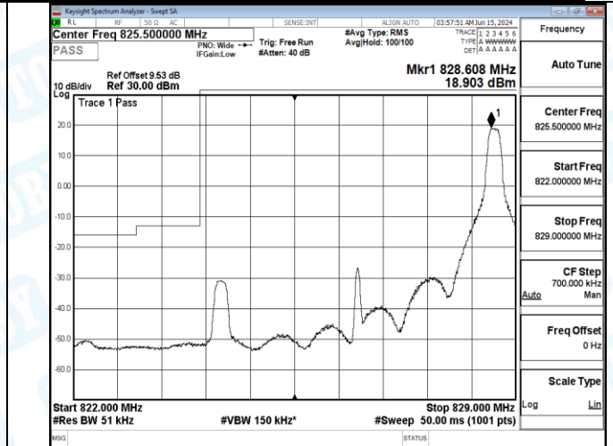
Band5_5MHz_QPSK_20625_1RB#0
