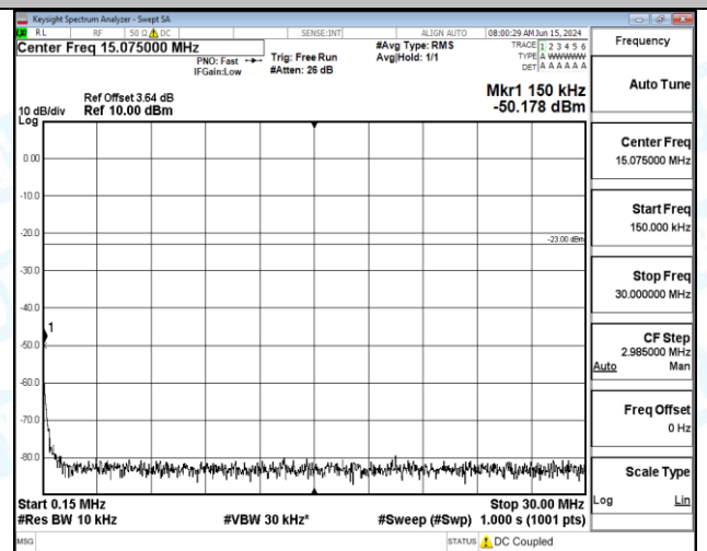
Band13_5MHz_QPSK_23255_25RB#0_1000~3000_1000~3000
