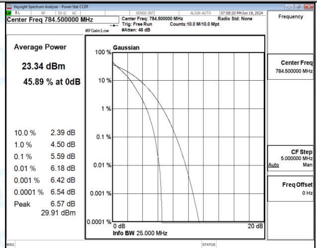
Band13-5MHz-16QAM-23205-25RB#0-PASS
