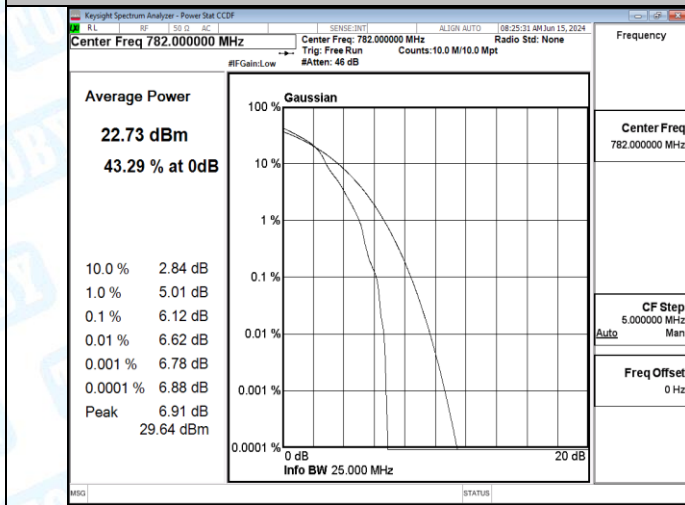
Band13-10MHz-16QAM-23230-1RB#0-PASS
