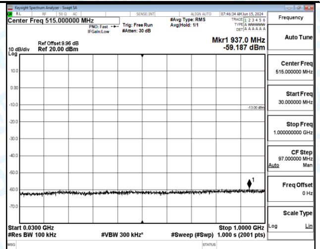
Band13_5MHz_QPSK_23205_1RB#24_3000~10000_3000~10000
