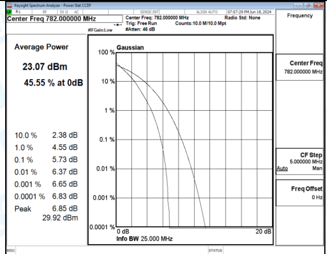
Band13-5MHz-QPSK-23255-25RB#0-PASS
