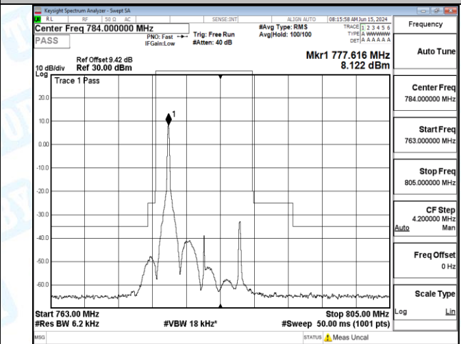
Band13_10MHz_16QAM_23230_1RB#0
