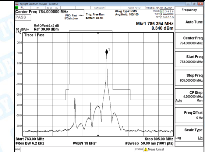
Band13_10MHz_16QAM_23230_1RB#0
