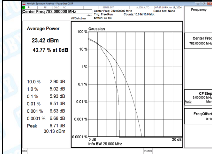
Band13-5MHz-16QAM-23255-1RB#0-PASS
