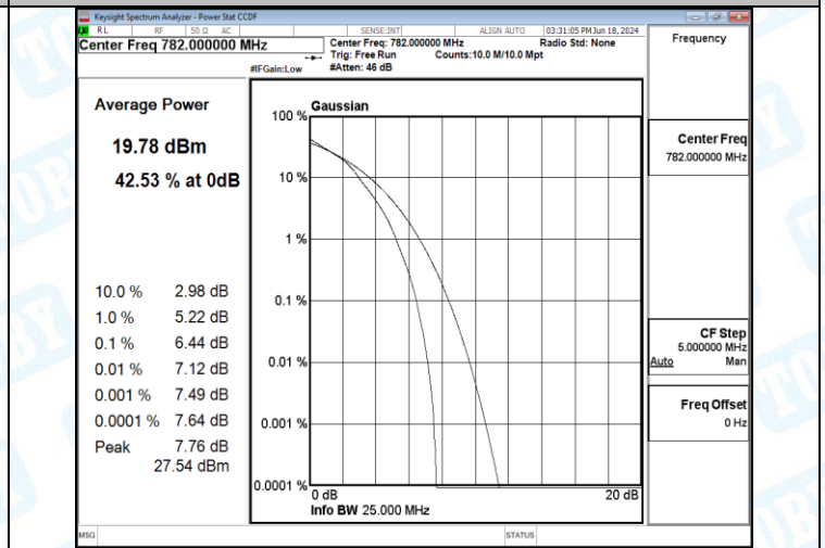
Band13-10MHz-16QAM-23230-27RB#0-PASS
