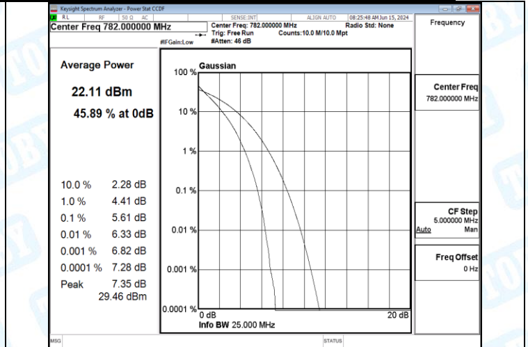
Band13-10MHz-16QAM-23230-27RB#0-PASS
