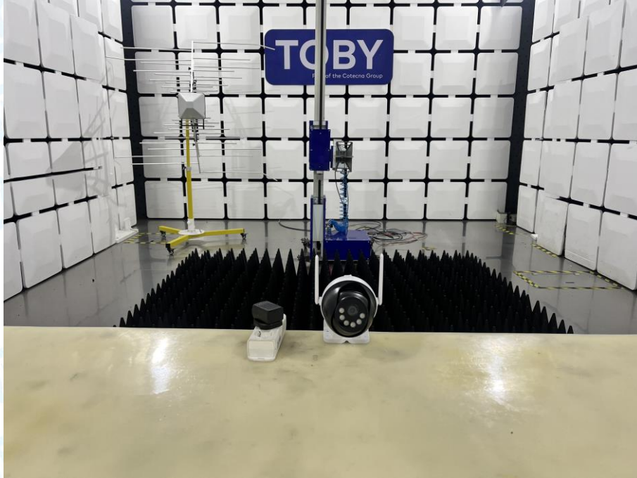
Photo of Setup for Radiated Emission (Above 1 GHz)-X10
