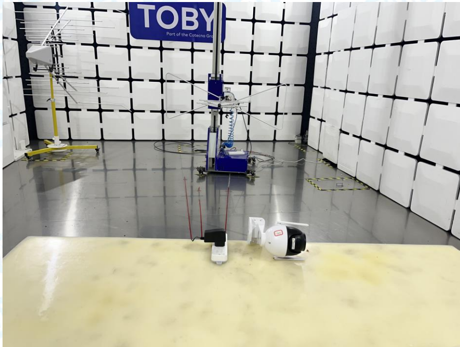
Photo of Setup for Radiated Emission (Below 1 GHz)-X20
