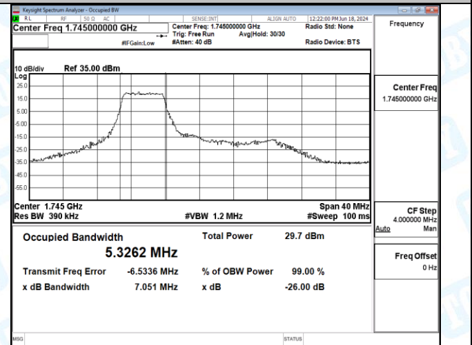
Band4-20MHz-16QAM-20300-27RB#0-PASS
