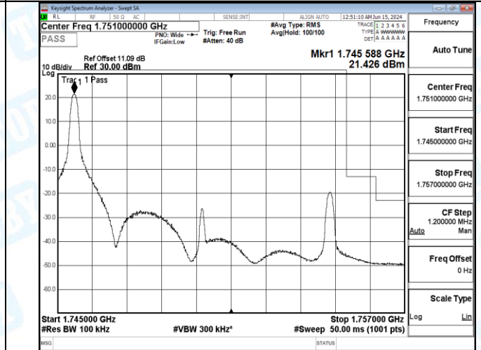
Band4_10MHz_QPSK_20350_50RB#0
