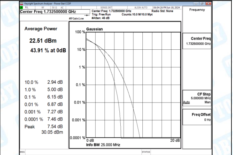
Band4-10MHz-16QAM-20350-27RB#0-PASS
