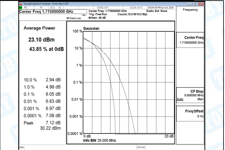
Band4-10MHz-16QAM-20175-27RB#0-PASS
