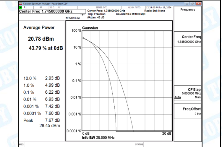
Band4-20MHz-16QAM-20300-27RB#0-PASS
