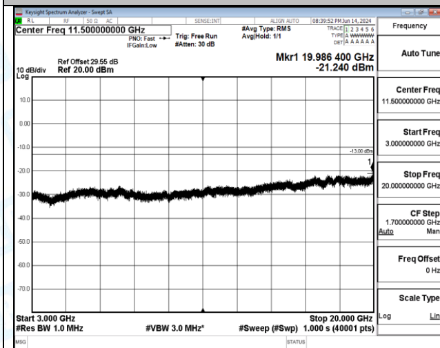
Band2_5MHz_QPSK_18625_1RB#24_0.15~30_0.15~30
