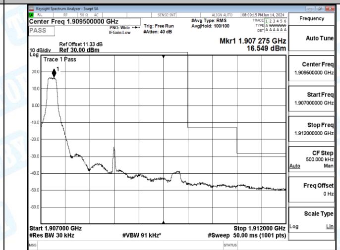
Band2_3MHz_QPSK_19185_15RB#0
