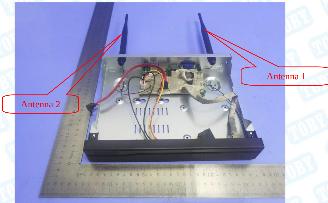
Photo 8 Internal of EUT
