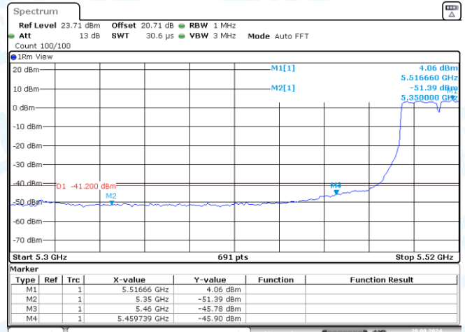
11N40SISO-Ant3-5510-PASS
