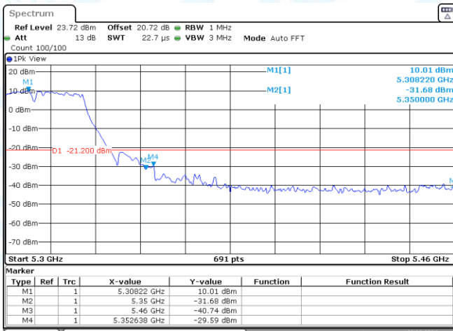
11N40SISO-Ant3-5190-PASS
