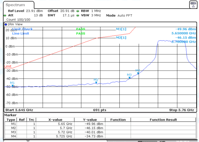
11A-Ant3-5745-PASS
