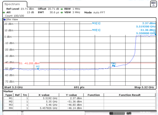
11AX40SISO-Ant3-5310-PASS
