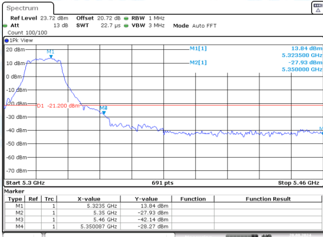
11N20SISO-Ant3-5320-PASS
