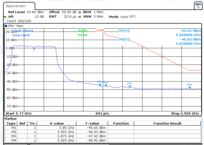
11N40SISO-Ant3-5755-PASS
