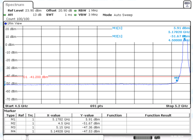
11AC20SISO-Ant3-5180-PASS
