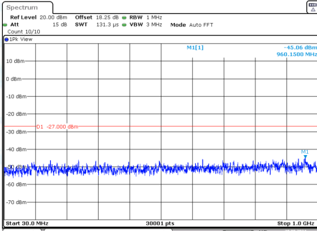
11AX40SISO-Ant3-5670-30~1000-PASS
