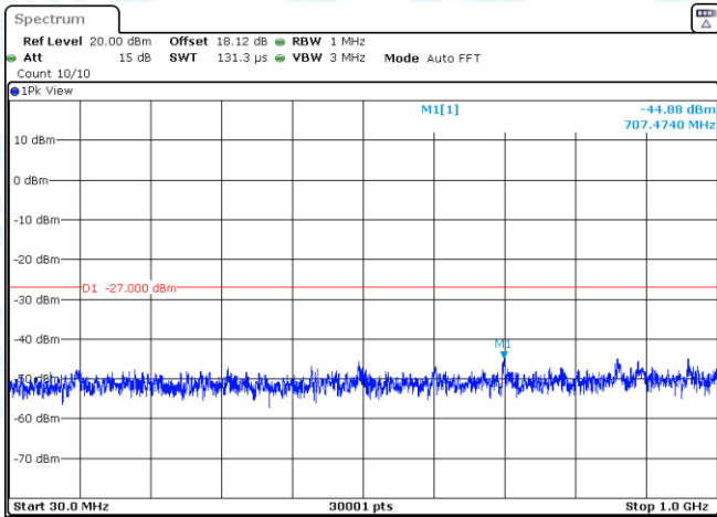
11AX40SISO-Ant3-5510-30~1000-PASS
