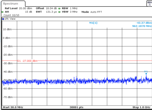
11AC40SISO-Ant3-5310-30~1000-PASS
