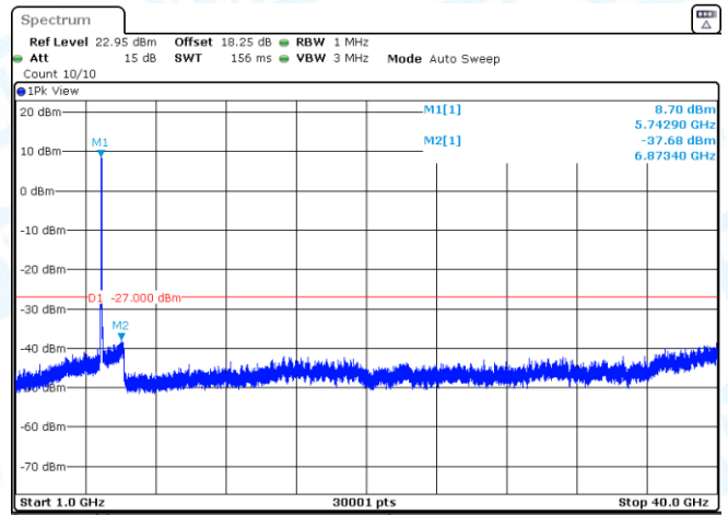
11AC40SISO-Ant3-5670-1000~40000-PASS
