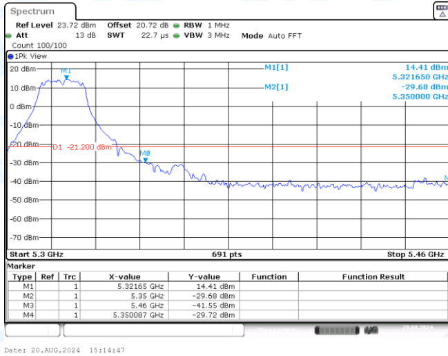
11A-Ant3-5320-PASS
