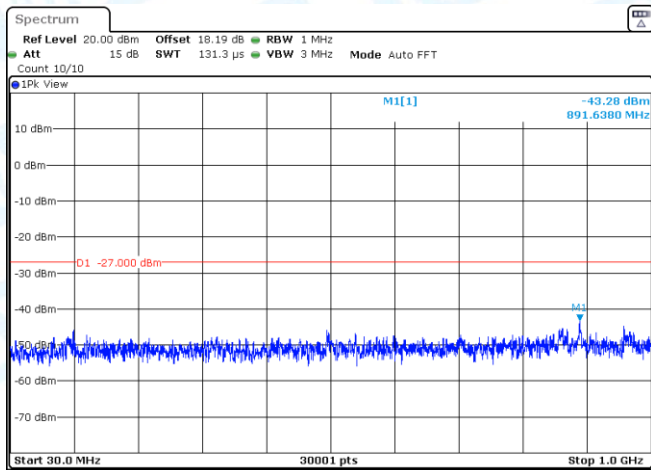
11AC40SISO-Ant3-5755-30~1000-PASS
