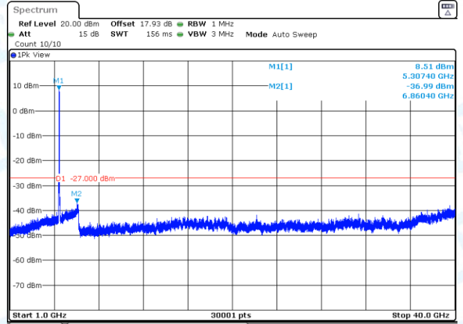
11AX40SISO-Ant3-5310-1000~40000-PASS
