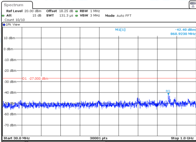
11AX20SISO-Ant3-5745-30~1000-PASS
