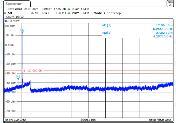
11AX20SISO-Ant3-5260-1000~40000-PASS
