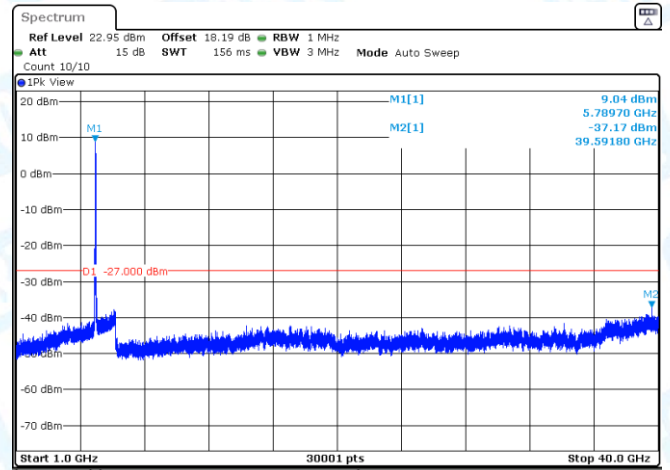
11AX40SISO-Ant3-5755-1000~40000-PASS
