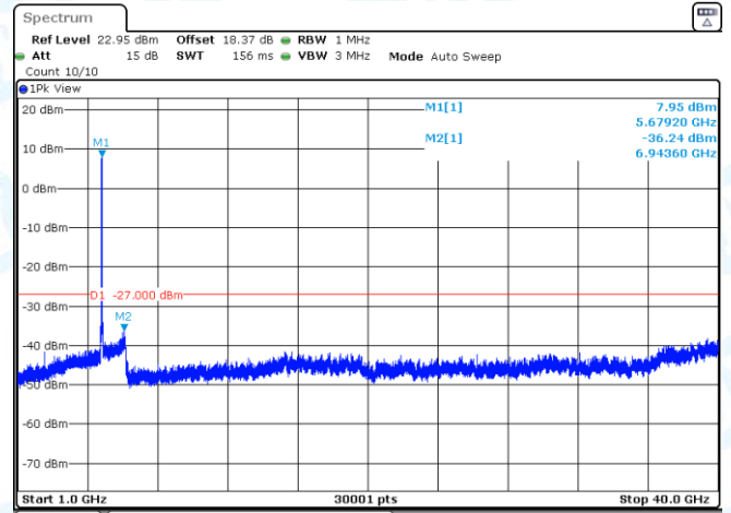
11AX40SISO-Ant3-5670-1000~40000-PASS
