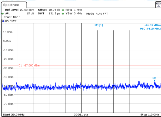
11AX20SISO-Ant3-5785-30~1000-PASS
