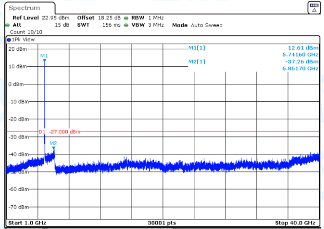
11AX20SISO-Ant3-5745-1000~40000-PASS
