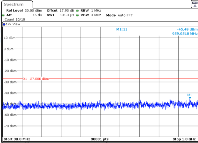
11AX40SISO-Ant3-5310-30~1000-PASS
