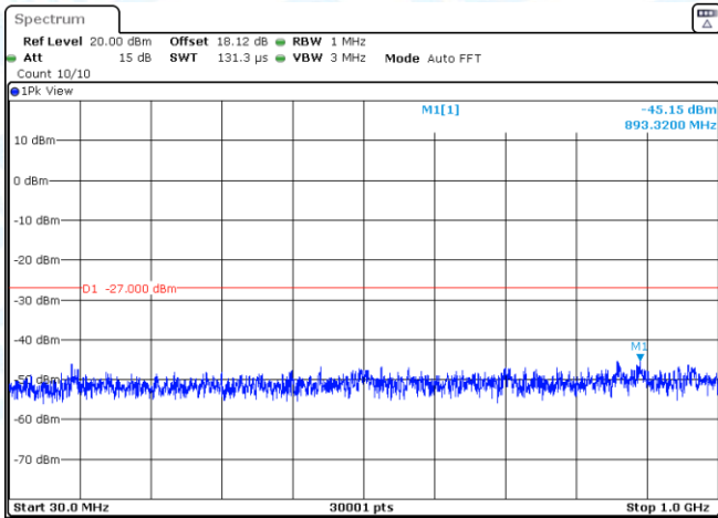
11AC40SISO-Ant3-5510-30~1000-PASS
