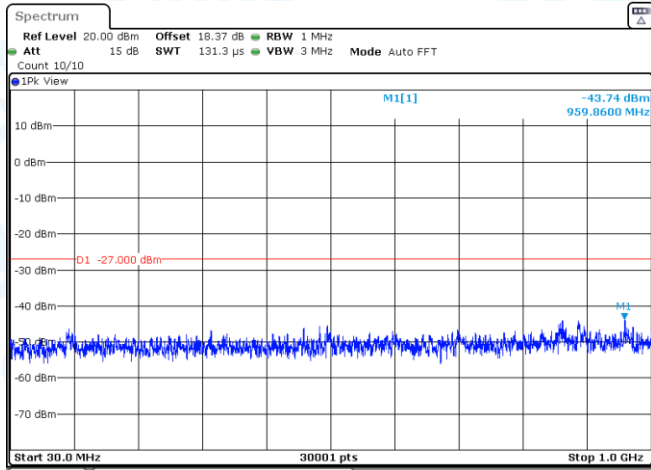
11AC40SISO-Ant3-5670-30~1000-PASS
