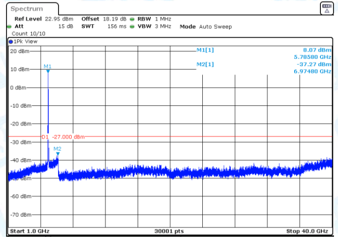
11N40SISO-Ant3-5755-1000~40000-PASS
