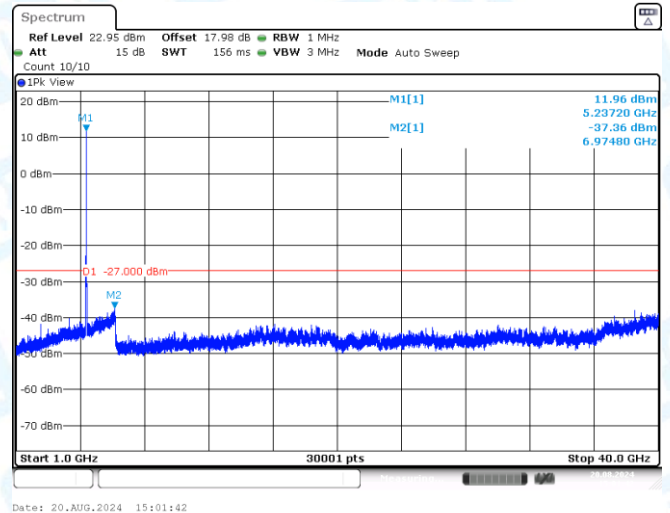
11A-Ant3-5240-1000~40000-PASS
