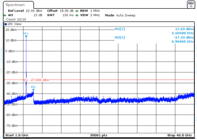
11N20SISO-Ant3-5500-1000~40000-PASS
