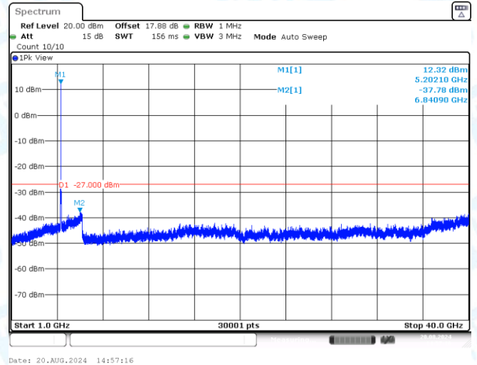
11A-Ant3-5200-1000~40000-PASS
