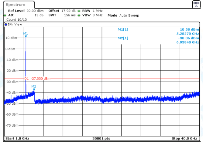
11N20SISO-Ant3-5260-1000~40000-PASS
