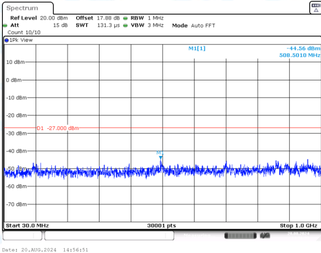
11A-Ant3-5200-30~1000-PASS
