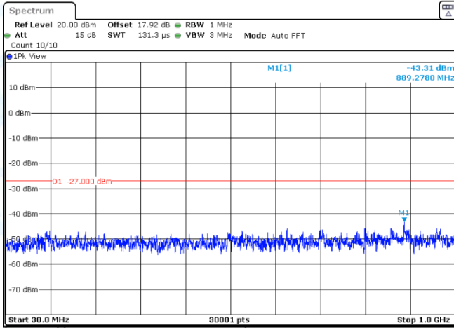
11N20SISO-Ant3-5260-30~1000-PASS
