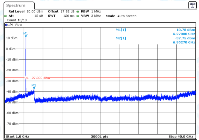
11AC20SISO-Ant3-5260-1000~40000-PASS
