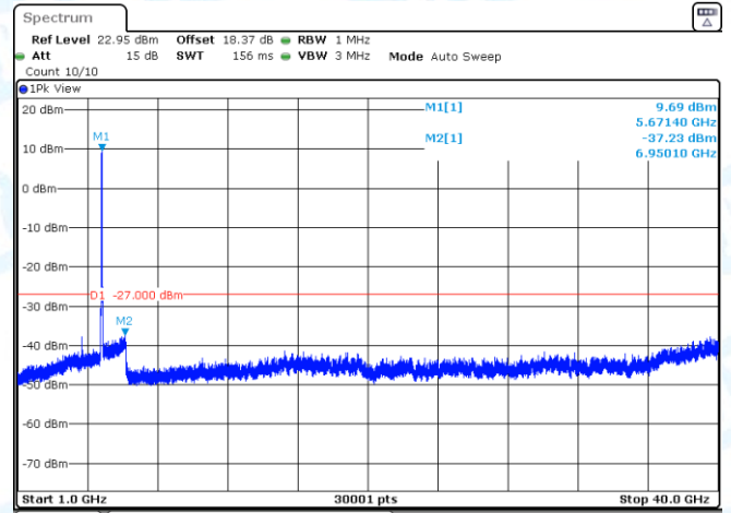
11N40SISO-Ant3-5670-1000~40000-PASS
