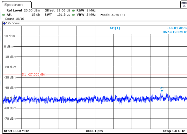
11AC20SISO-Ant3-5500-30~1000-PASS
