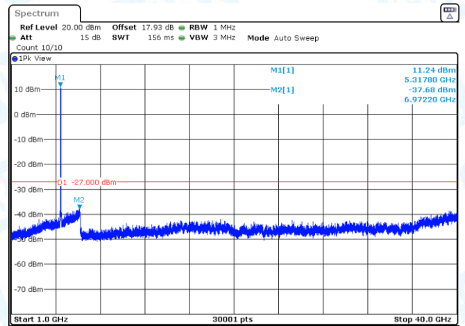
11AC20SISO-Ant3-5280-1000~40000-PASS
