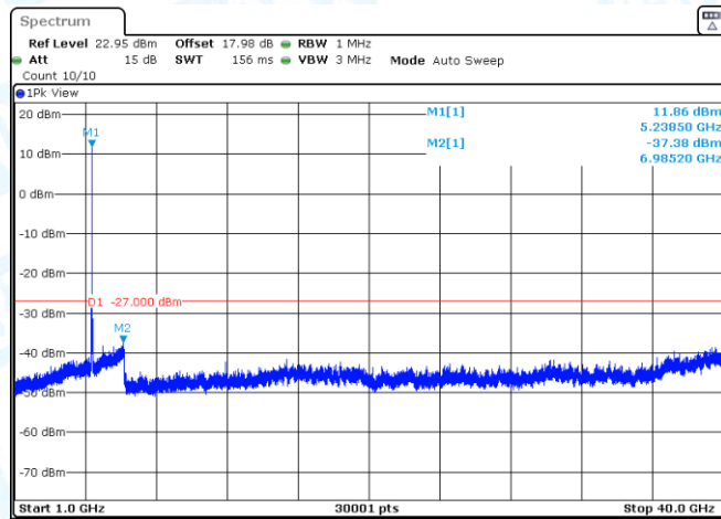
11N20SISO-Ant3-5200-1000~40000-PASS
