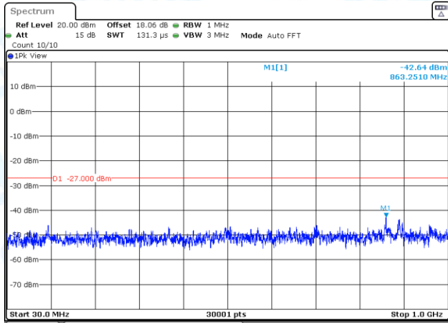
11N20SISO-Ant3-5500-30~1000-PASS
