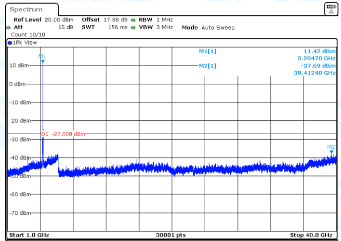
11AC20SISO-Ant3-5180-1000~40000-PASS
