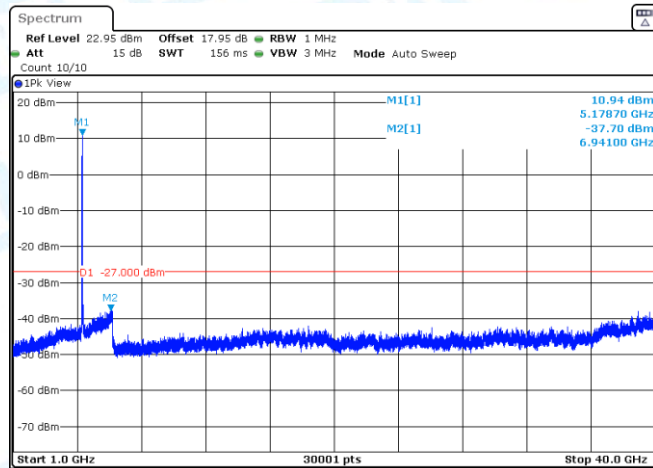
11N20SISO-Ant3-5180-1000~40000-PASS
