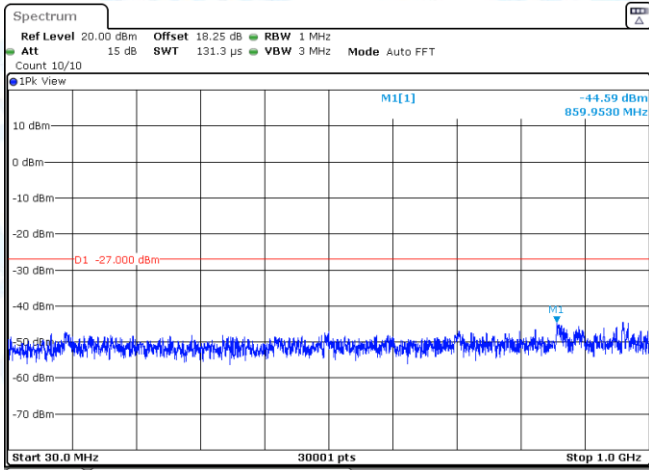
11N20SISO-Ant3-5745-30~1000-PASS
