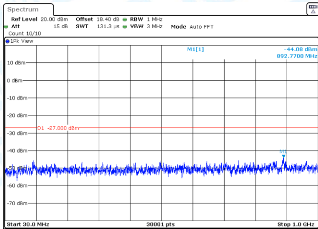
11N20SISO-Ant3-5580-30~1000-PASS
