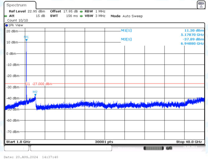
11A-Ant3-5180-1000~40000-PASS
