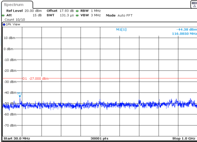
11N20SISO-Ant3-5280-30~1000-PASS
