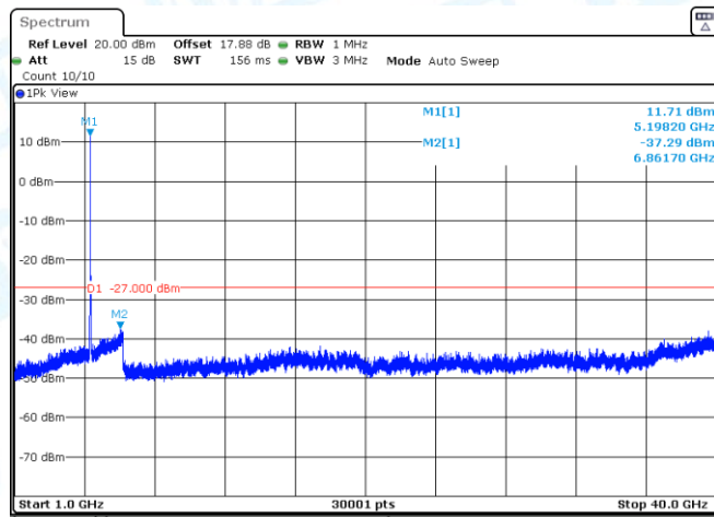
11N20SISO-Ant3-5180-1000~40000-PASS
