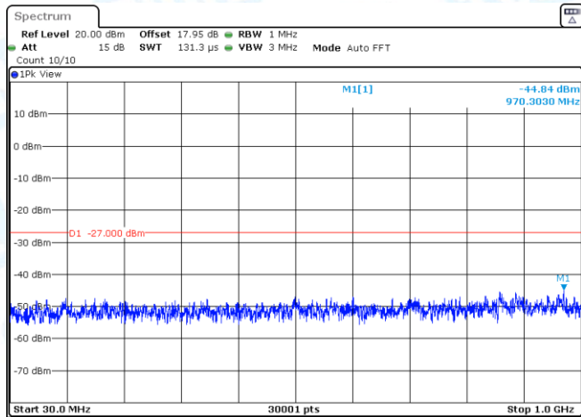
11N20SISO-Ant3-5180-30~1000-PASS
