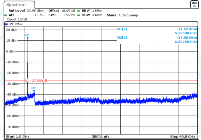
11A-Ant3-5500-1000~40000-PASS
