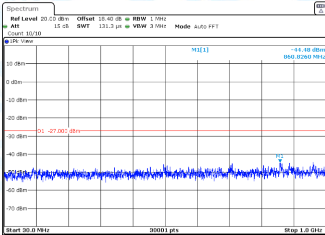
11A-Ant3-5580-30~1000-PASS
