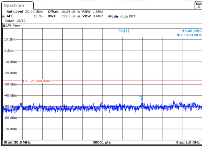
11N20SISO-Ant3-5785-30~1000-PASS
