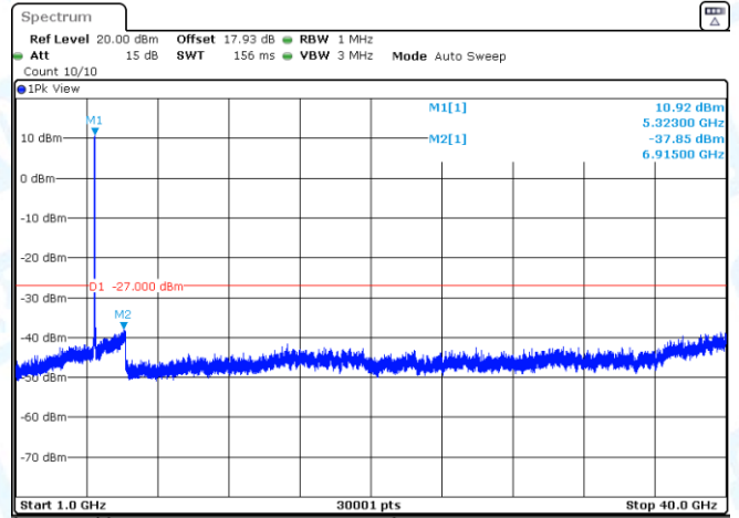
11N20SISO-Ant3-5280-1000~40000-PASS
