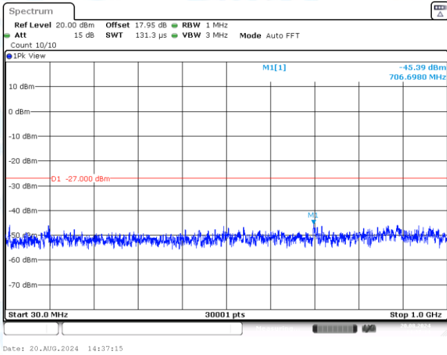
11A-Ant3-5180-30~1000-PASS
