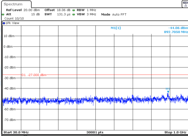
11A-Ant3-5500-30~1000-PASS
