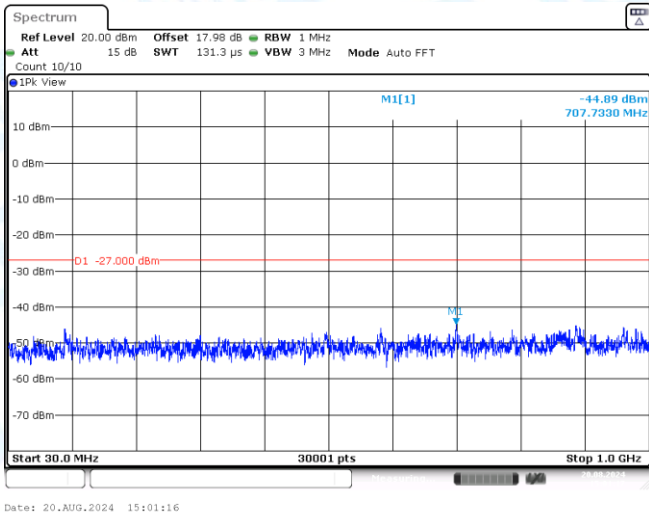
11A-Ant3-5240-30~1000-PASS
