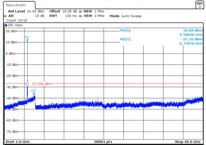
11AC20SISO-Ant3-5500-1000~40000-PASS
