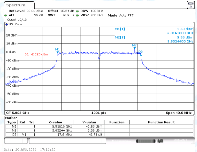
11N20SISO-Ant3-5825-PASS
