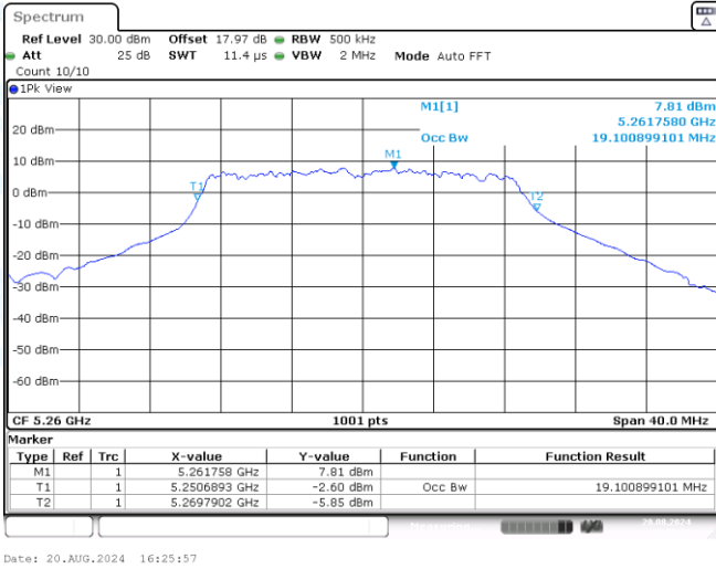
11N20SISO-Ant3-5260
