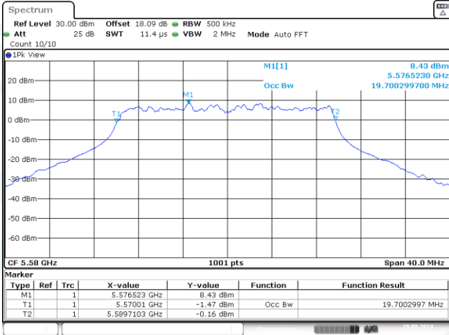
11AX20ISO-Ant3-5580
