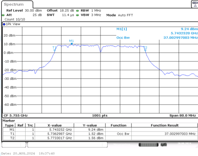
11N40SISO-Ant3-5755
