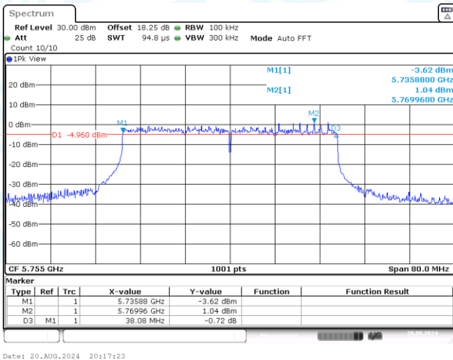
11AC40SISO-Ant3-5755-PASS
