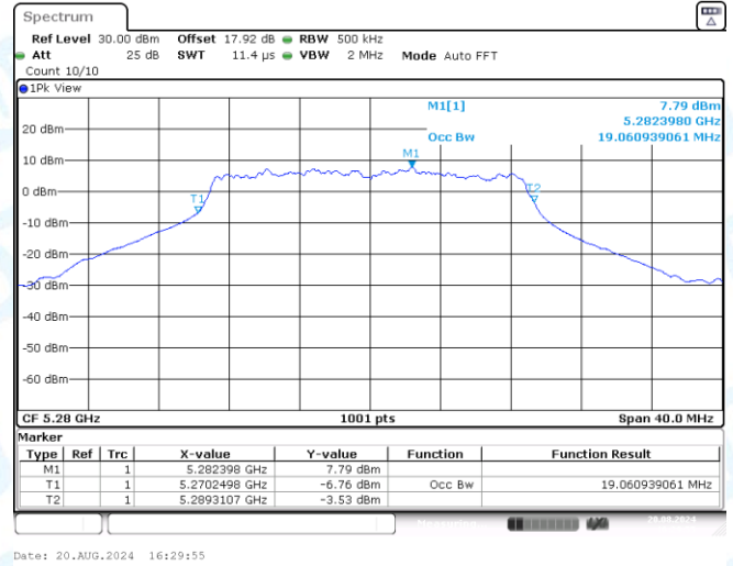
11N20SISO-Ant3-5280
