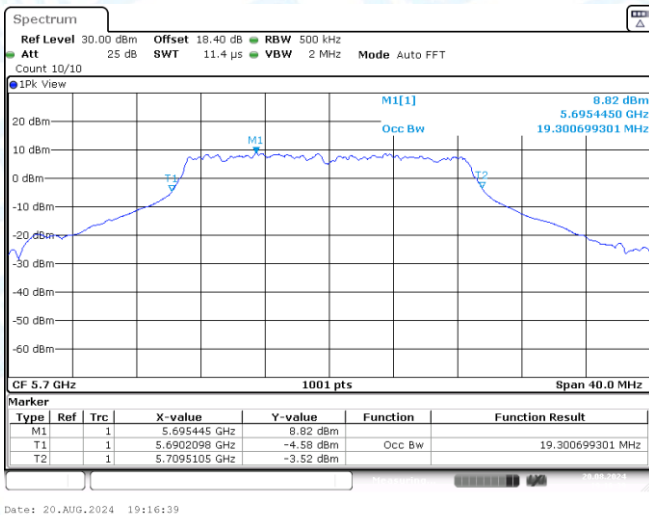
11AC20SISO-Ant3-5700
