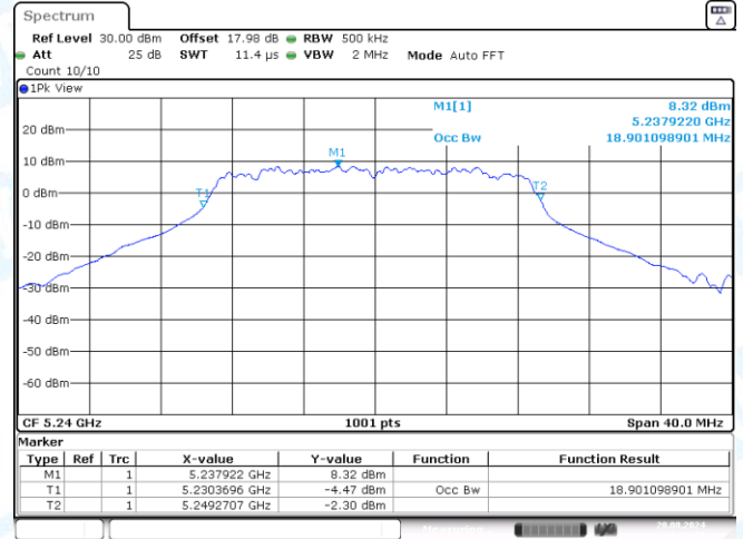
11N20SISO-Ant3-5240
