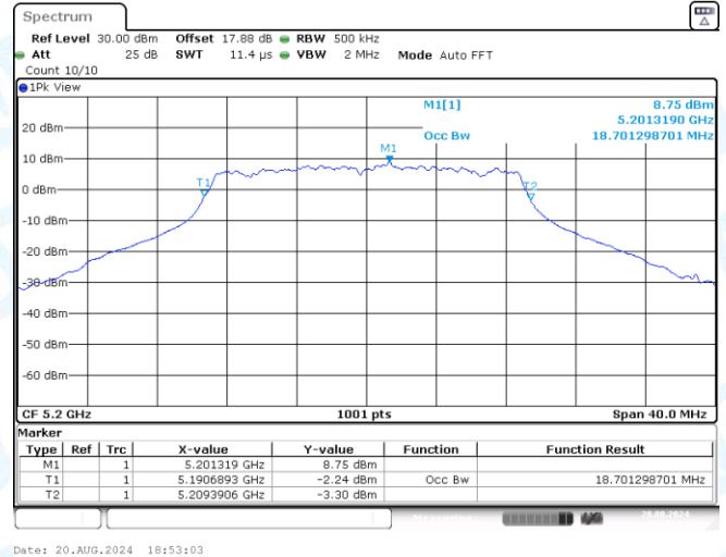
11AC20SISO-Ant3-5200
