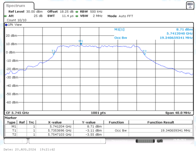
11AC20SISO-Ant3-5745
