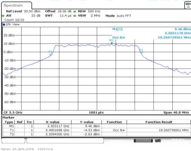
11AC20SISO-Ant3-5500
