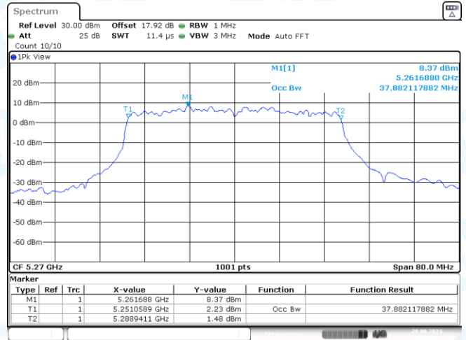
11AX40SISO-Ant3-5270
