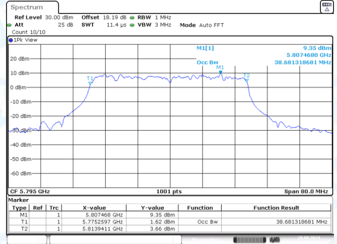
11AX40SISO-Ant3-5795
