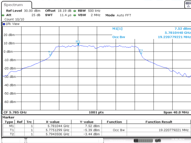
11AC20SISO-Ant3-5785
