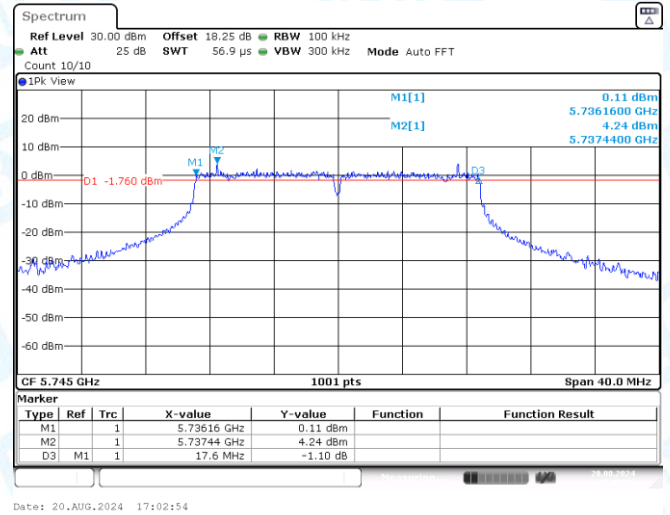
11N20SISO-Ant3-5745-PASS
