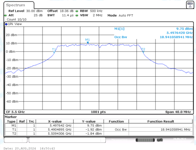
11N20SISO-Ant3-5500
