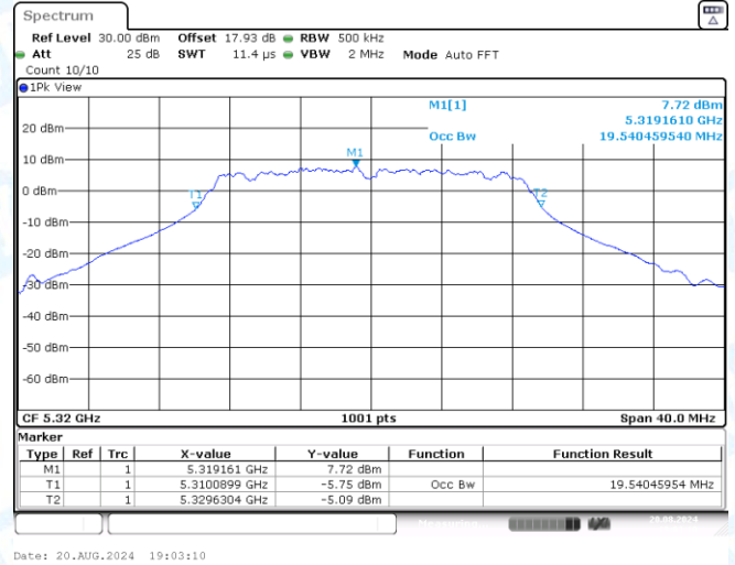
11AC20SISO-Ant3-5320
