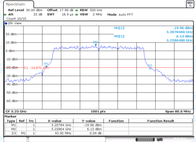
11AX40SISO-Ant3-5230
