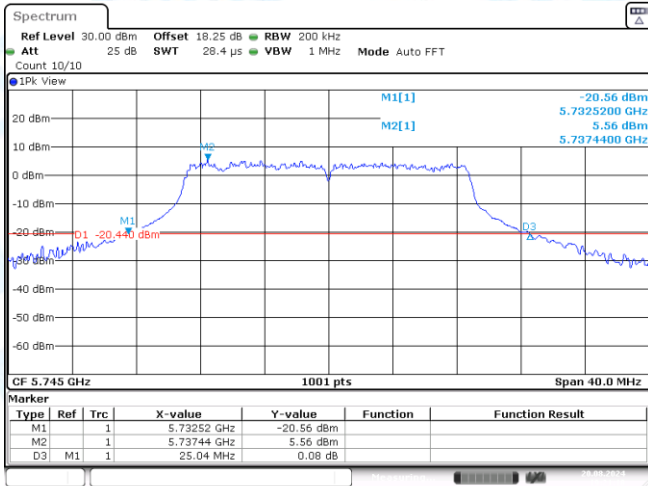
11AC20ISO-Ant3-5745
