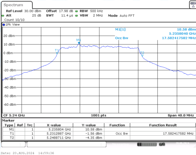
11A-Ant3-5240
