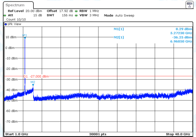
11AC40SISO-Ant2-5230-1000~40000-PASS
