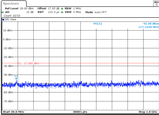
11AC40SISO-Ant2-5310-30~1000-PASS
