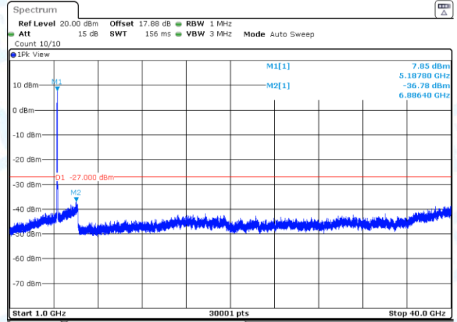
11AX40SISO-Ant2-5190-1000~40000-PASS
