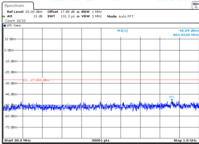
11AX20SISO-Ant2-5180-30~1000-PASS
