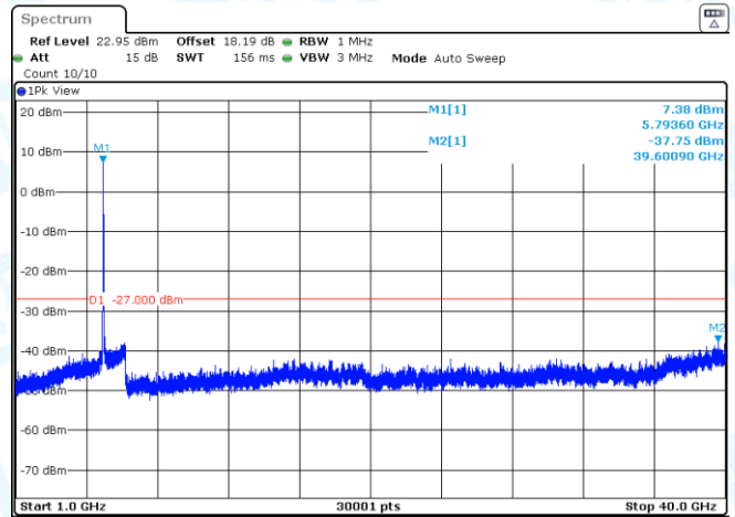
11AC40SISO-Ant2-5755-1000~40000-PASS
