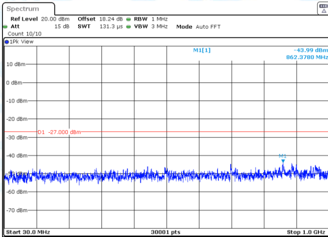
11AX20SISO-Ant2-5785-30~1000-PASS
