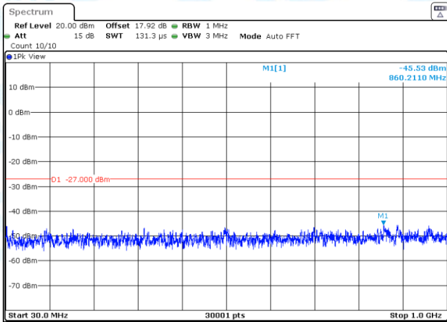
11AC40SISO-Ant2-5230-30~1000-PASS
