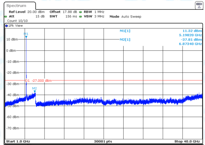
11AX20SISO-Ant2-5180-1000~40000-PASS
