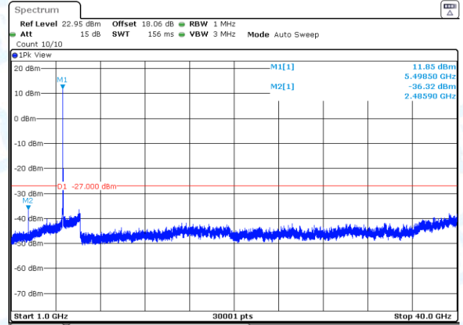
11AX20SISO-Ant2-5500-1000~40000-PASS
