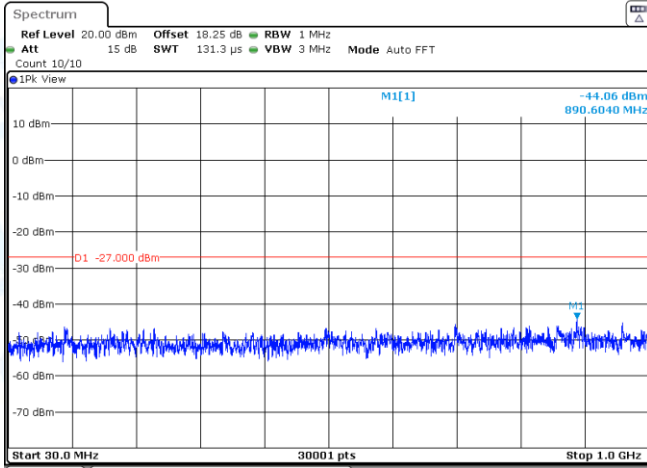
11AX20SISO-Ant2-5745-30~1000-PASS
