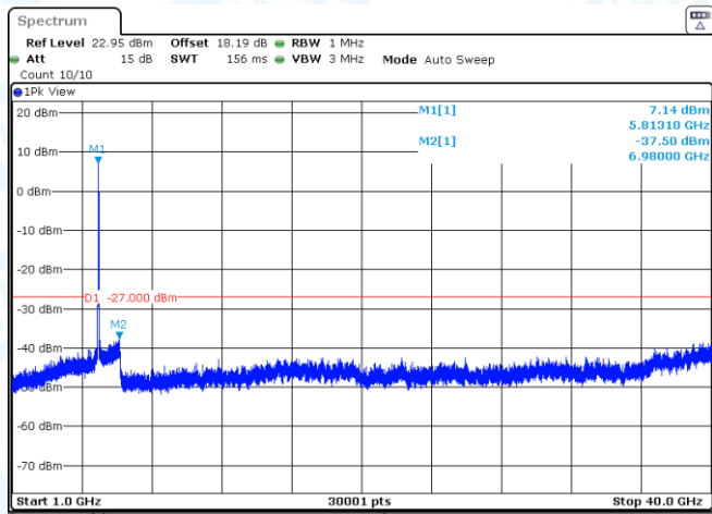
11AX40SISO-Ant2-5755-1000~40000-PASS
