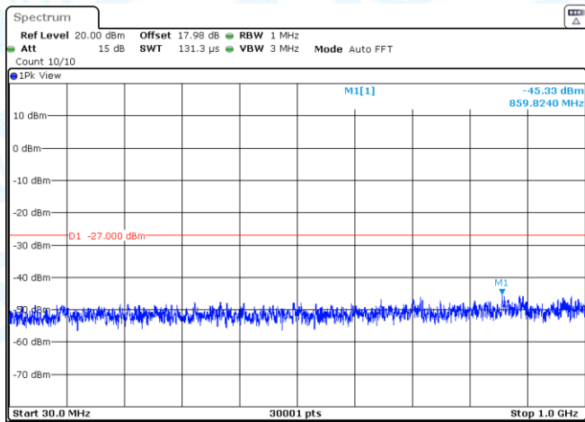
11AX20SISO-Ant2-5200-30~1000-PASS
