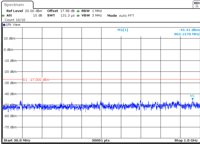
11AC40SISO-Ant2-5190-30~1000-PASS
