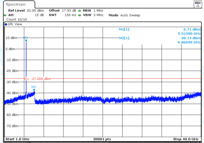
11AC40SISO-Ant2-5310-1000~40000-PASS
