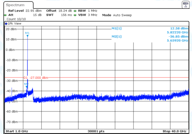
11AX20SISO-Ant2-5785-1000~40000-PASS
