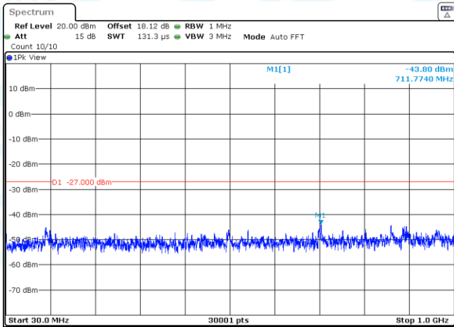
11AC40SISO-Ant2-5510-30~1000-PASS
