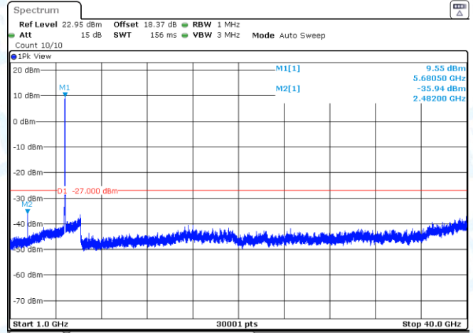
11AC40SISO-Ant2-5670-1000~40000-PASS
