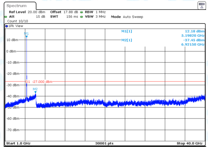
11N20SISO-Ant2-5180-1000~40000-PASS
