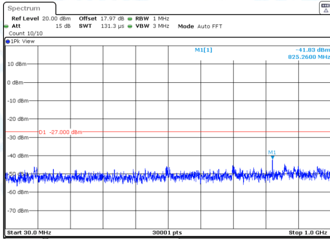
11A-Ant2-5260-30~1000-PASS
