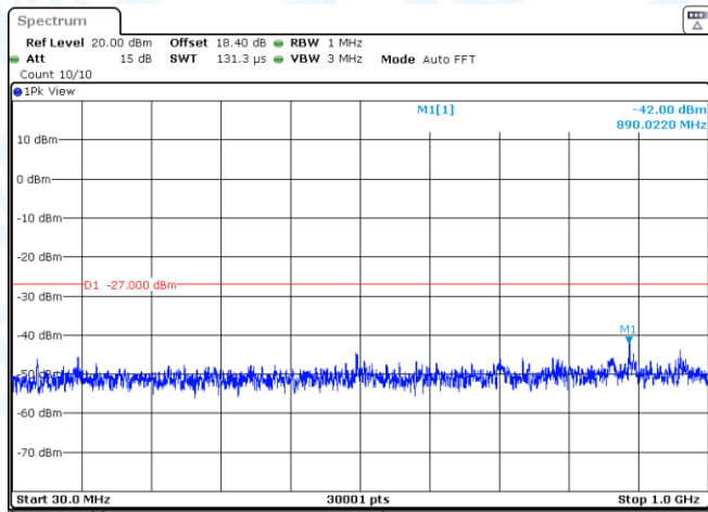
11AC20SISO-Ant2-5580-30~1000-PASS
