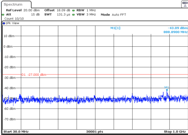
11A-Ant2-5500-30~1000-PASS
