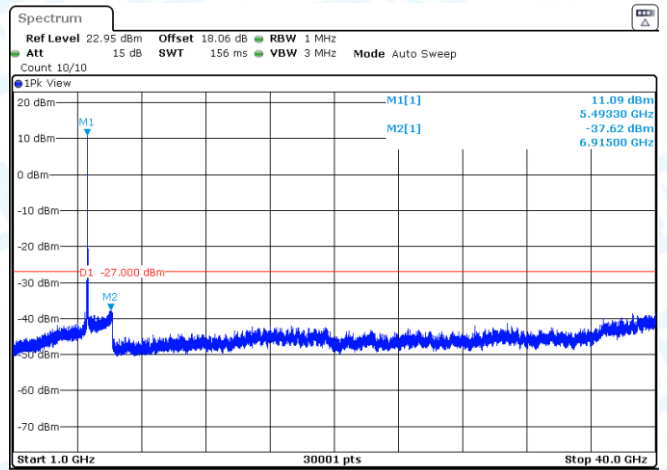
11N20SISO-Ant2-5500-1000~40000-PASS
