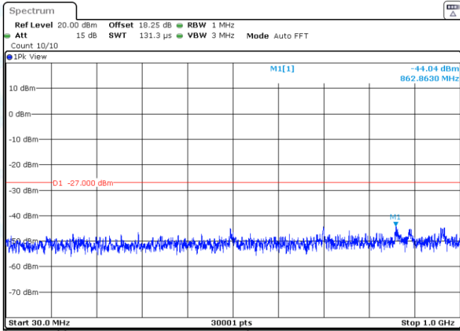
11N40SISO-Ant2-5670-30~1000-PASS
