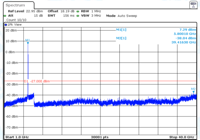
11N40SISO-Ant2-5755-1000~40000-PASS
