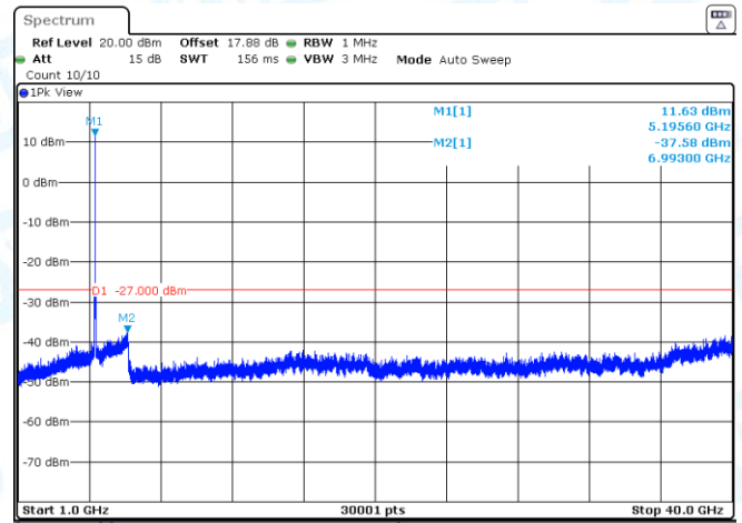
11AC20SISO-Ant2-5180-1000~40000-PASS
