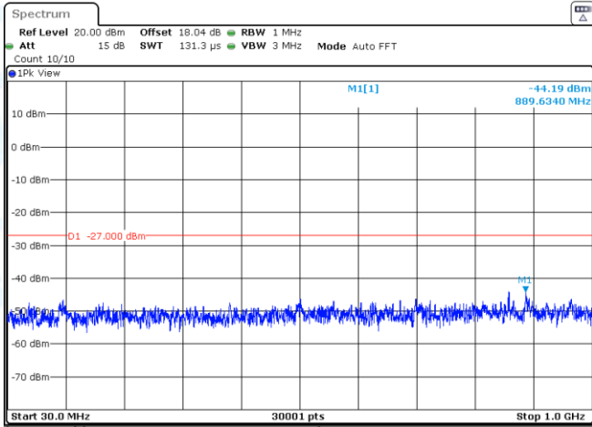
11N40SISO-Ant2-5310-30~1000-PASS
