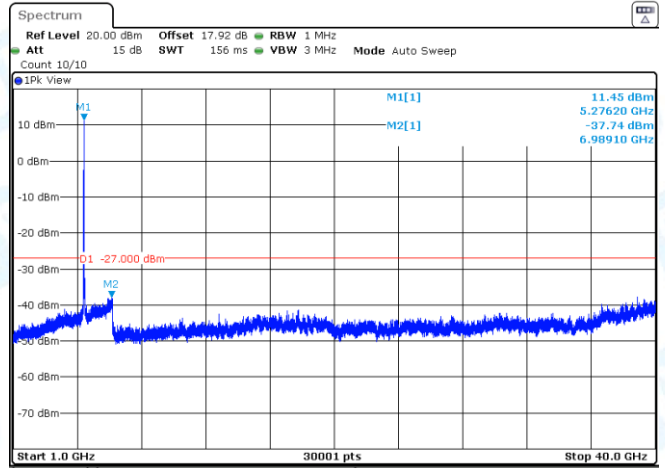
11AC20SISO-Ant2-5260-1000~40000-PASS
