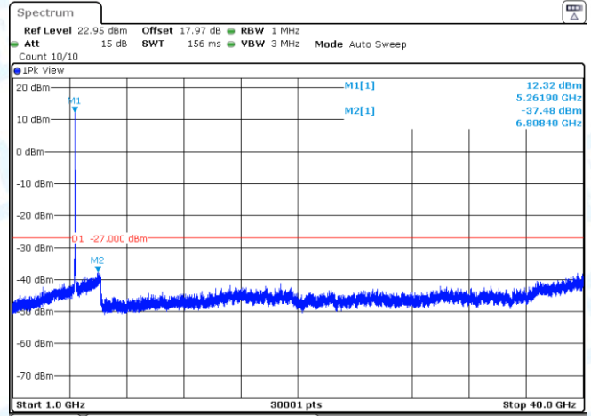
11N20SISO-Ant2-5260-1000~40000-PASS
