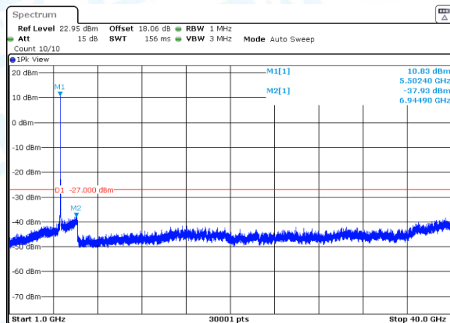
11AC20SISO-Ant2-5500-1000~40000-PASS
