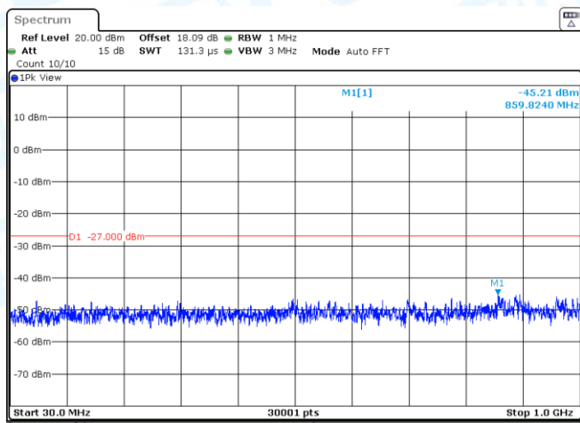
11AC20SISO-Ant2-5500-30~1000-PASS
