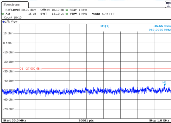
11N40SISO-Ant2-5755-30~1000-PASS
