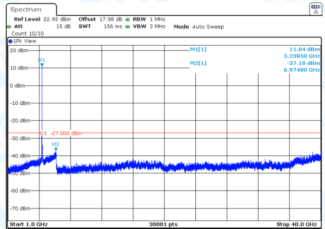
11AC20SISO-Ant2-5200-1000~40000-PASS
