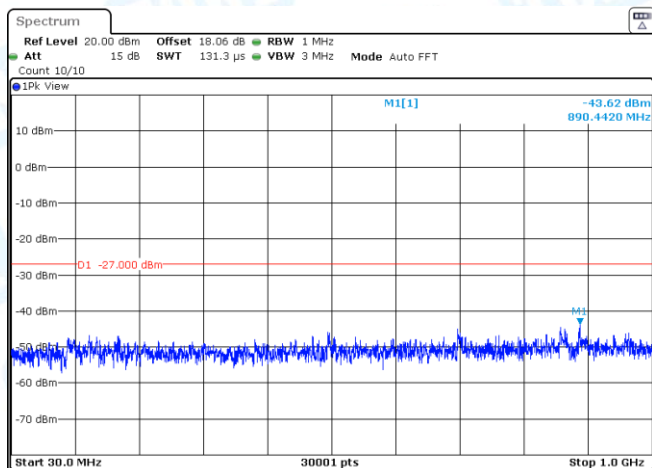
11AC20SISO-Ant2-5500-30~1000-PASS
