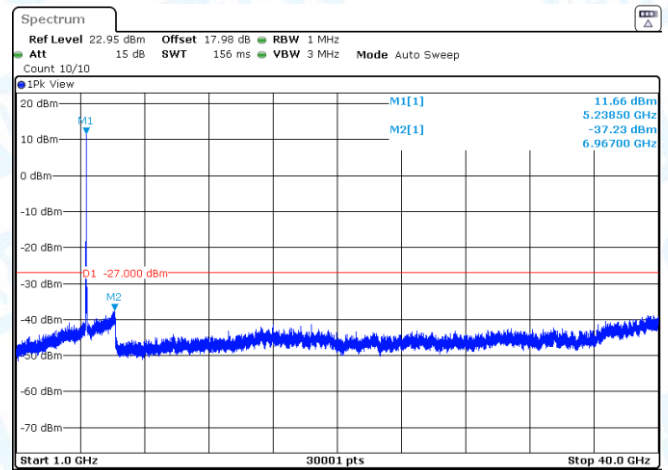
11N20SISO-Ant2-5200-1000~40000-PASS
