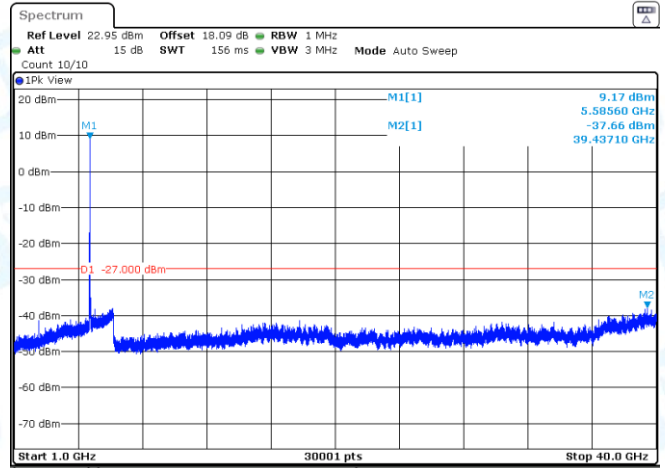
11A-Ant2-5500-1000~40000-PASS
