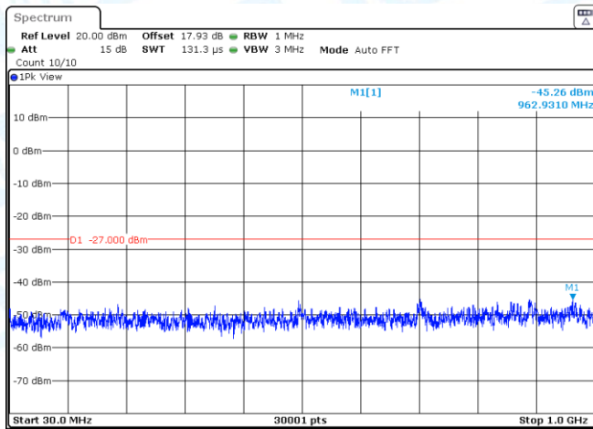
11A-Ant2-5280-30~1000-PASS
