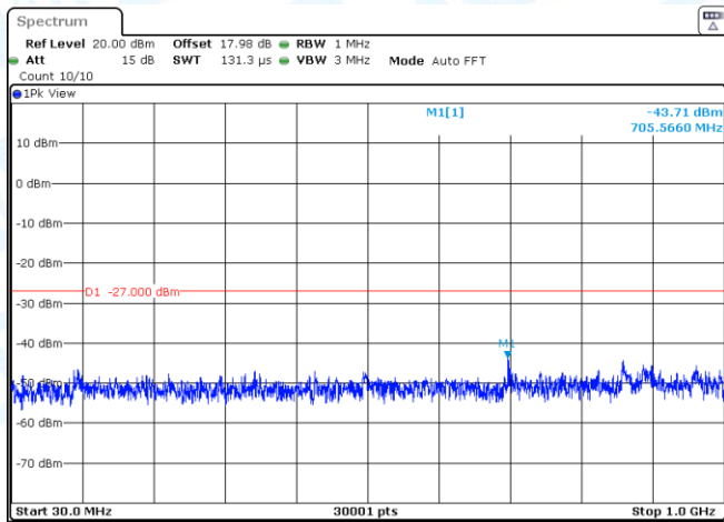
11AC20SISO-Ant2-5200-30~1000-PASS
