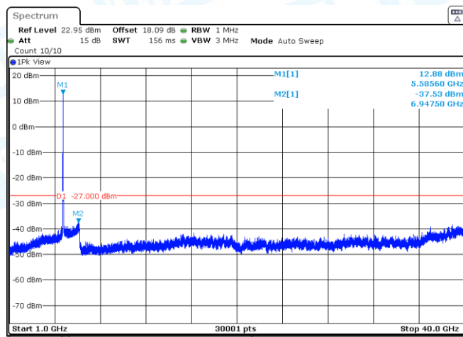
11AC20SISO-Ant2-5500-1000~40000-PASS
