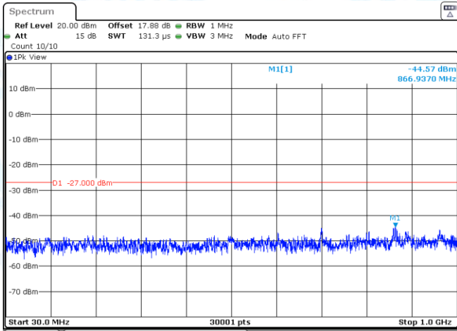
11N40SISO-Ant2-5190-30~1000-PASS
