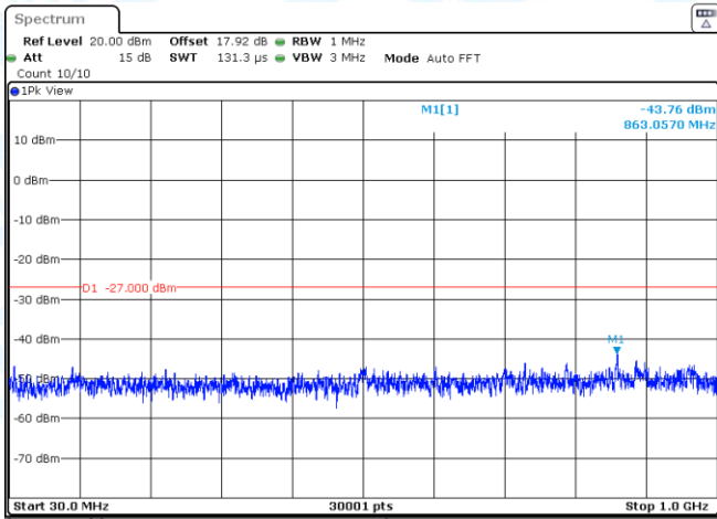
11N40SISO-Ant2-5230-30~1000-PASS
