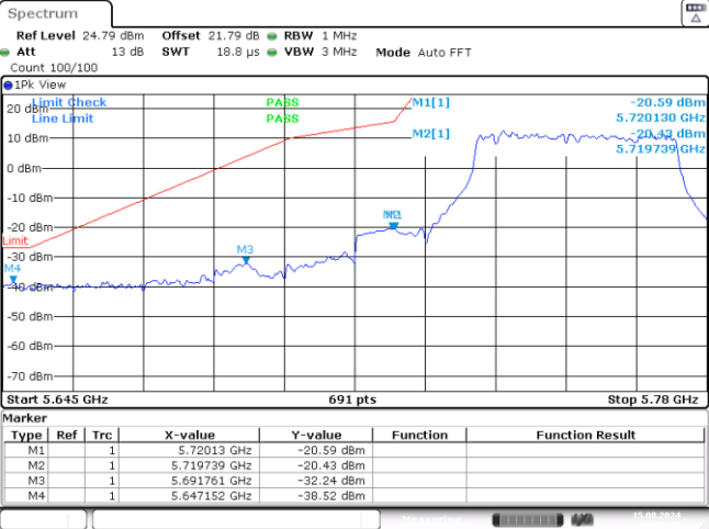
11AX40SISO-Ant2-5755-PASS
