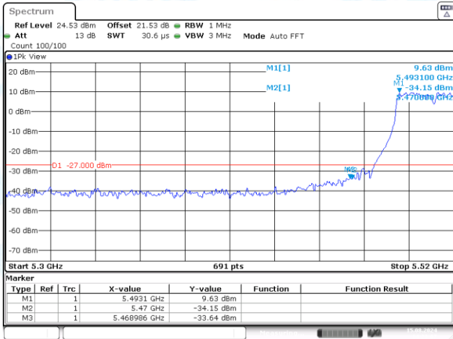
11AC40SISO-Ant2-5510-PASS
