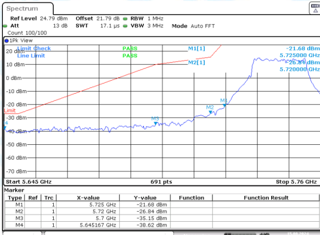
11AC40SISO-Ant2-5755-PASS
