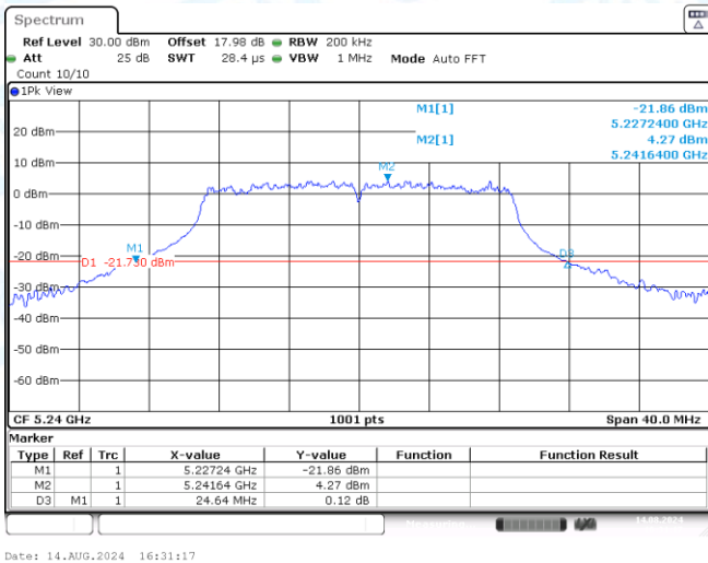
11N20SISO-Ant2-5240
