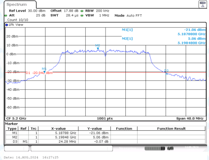
11N20SISO-Ant2-5200
