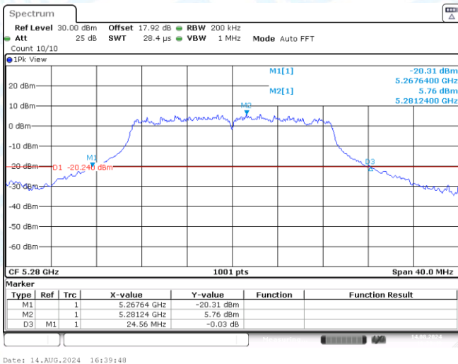
11N20SISO-Ant2-5280
