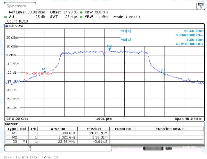
11N20SISO-Ant2-5320
