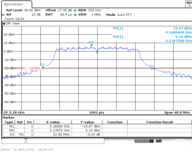
11N20SISO-Ant2-5180
