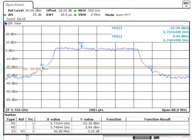
11N40SISO-Ant2-5755
