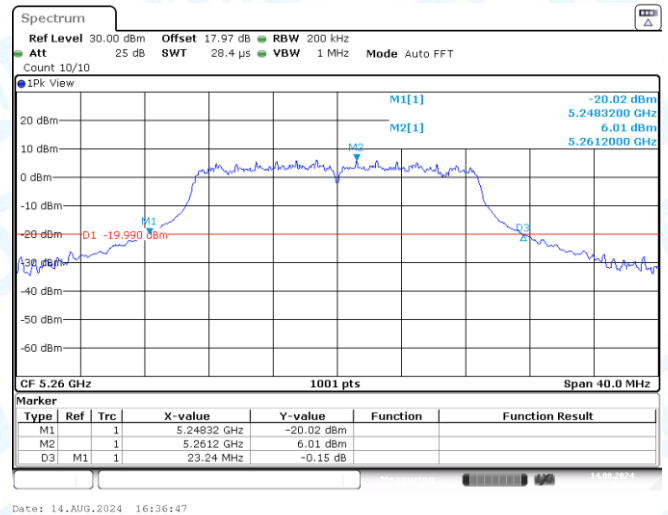
11N20SISO-Ant2-5260
