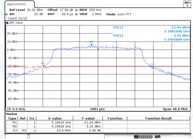
11AX20SISO-Ant2-5200
