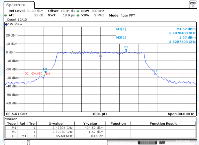
11AC40SISO-Ant2-5510
