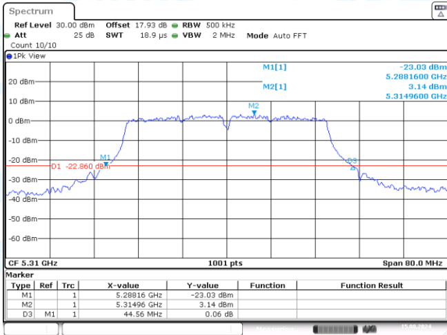
11AC40SISO-Ant2-5310
