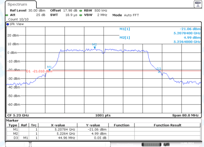
11N40SISO-Ant2-5230
