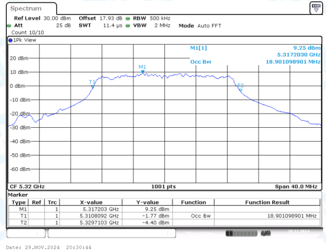
11N20SISO-Ant1-5320
