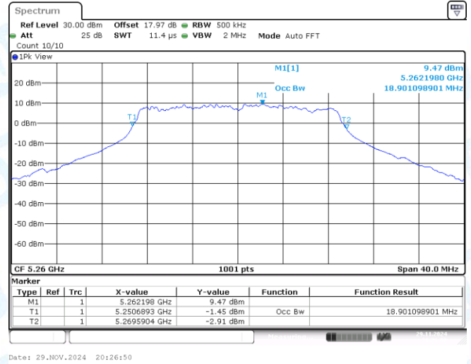
11N20SISO-Ant1-5260
