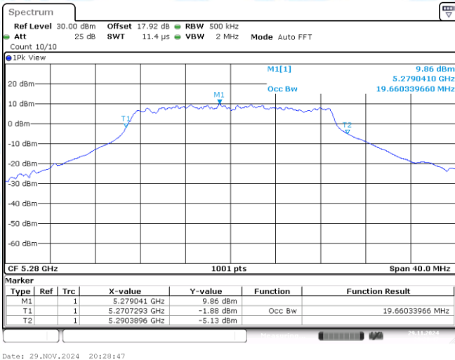
11N20SISO-Ant1-5280
