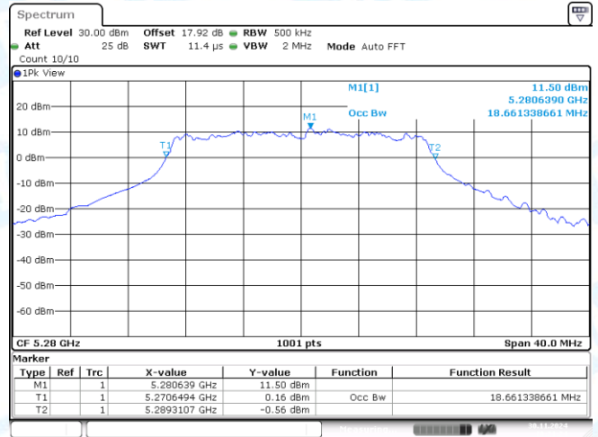
11AC20SISO-Ant1-5280
