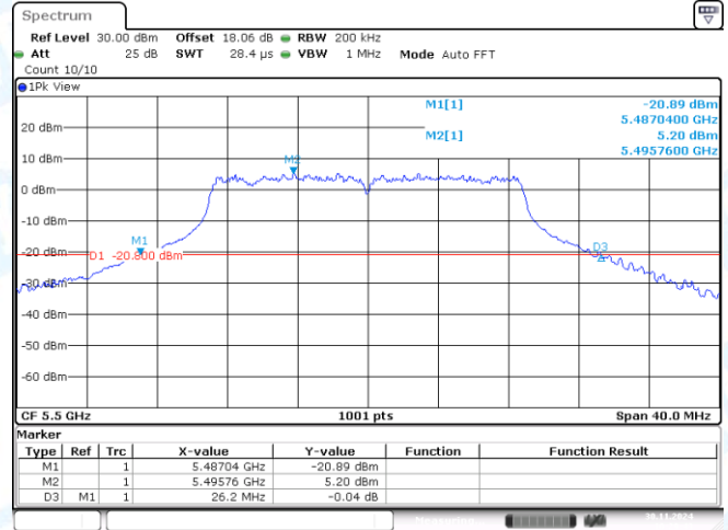
11AC20SISO-Ant1-5500
