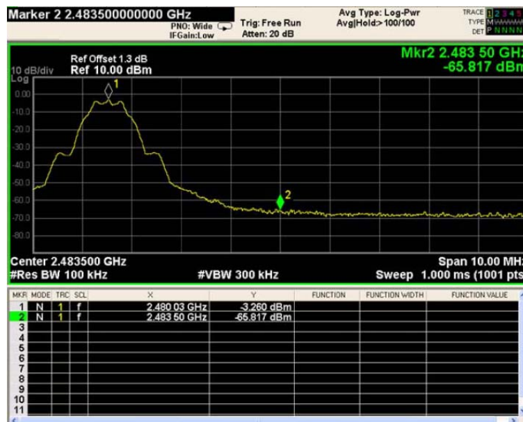
High Band Edge Plot on Channel 39
