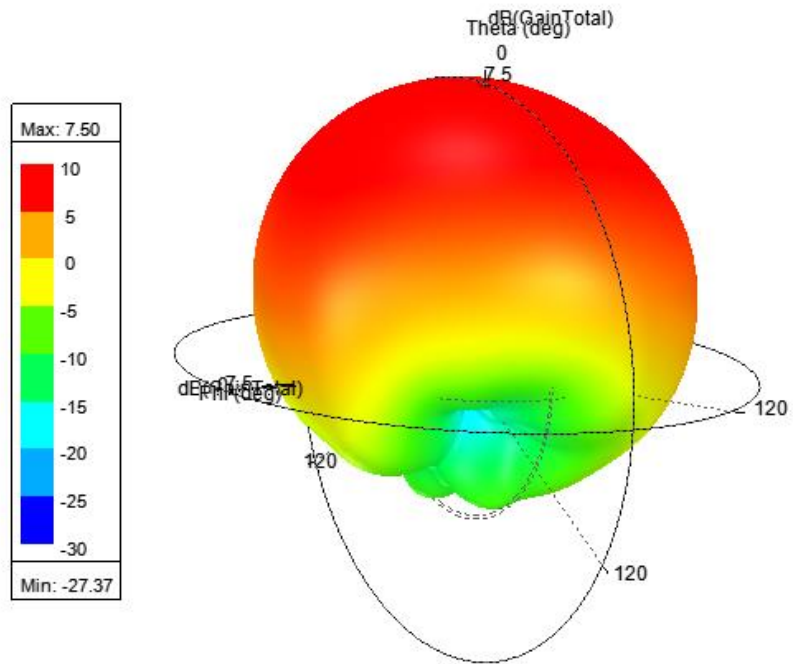
3D patterns @5.1GHz @ ANT 3
