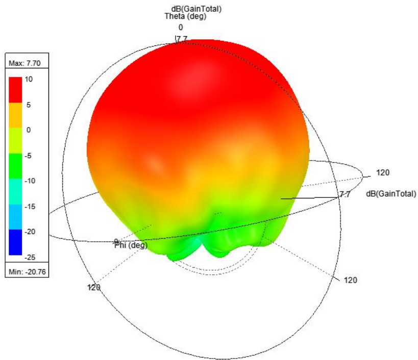
3D patterns @5.5GHz @ ANT 3
