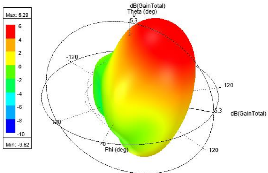
3D patterns @2.5GHz @ ANT 1/@ ANT 2
