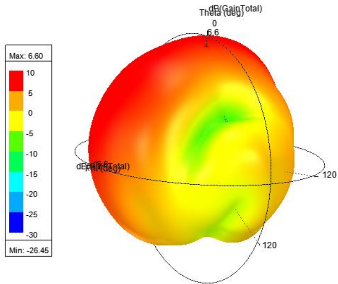
3D patterns @5.5GHz @ ANT 1/2
