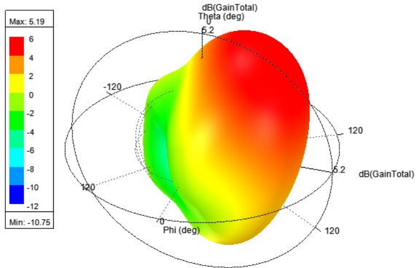
3D patterns @2.4GHz @ ANT 1/@ ANT 2
