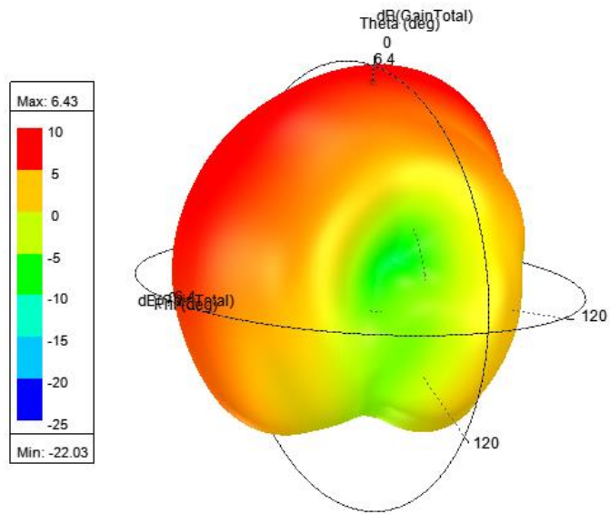
3D patterns @5.1GHz @ ANT 1/@ ANT 2
