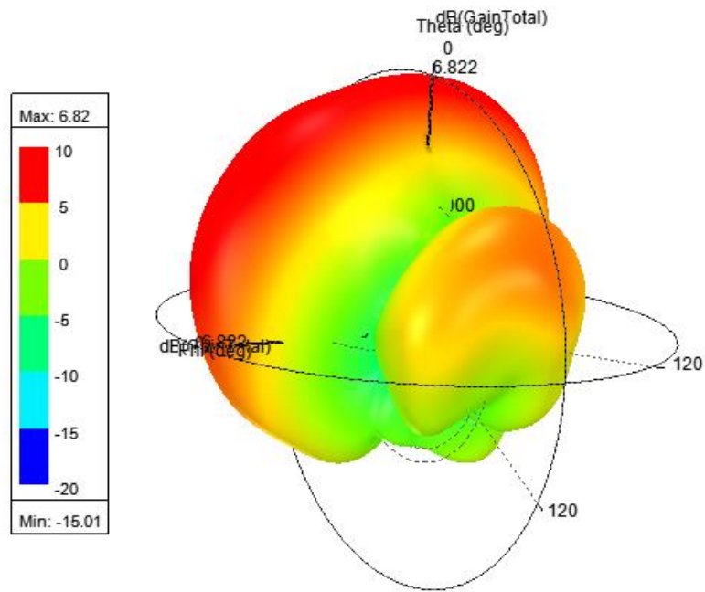
3D patterns @5.9GHz @ ANT 1/2
