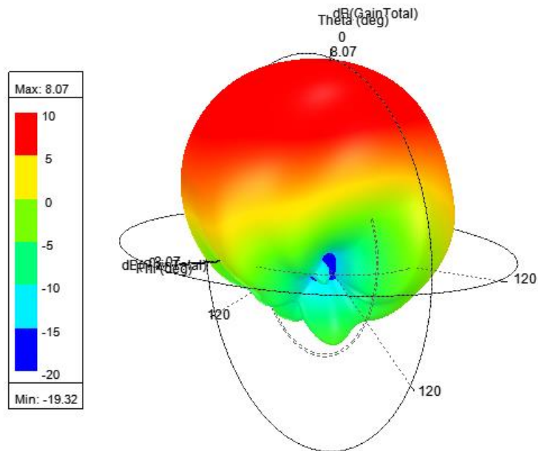
3D patterns @5.9GHz @ ANT 3
