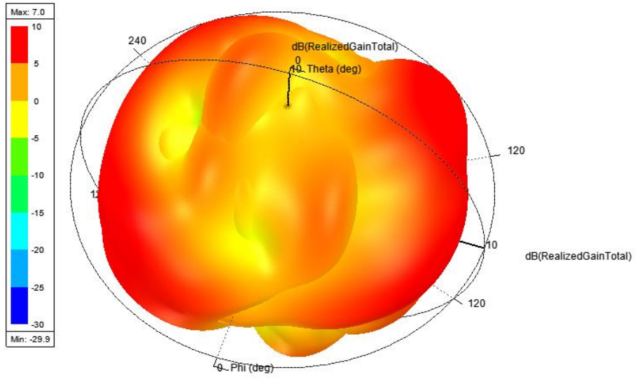
3D patterns @5.9GHz
